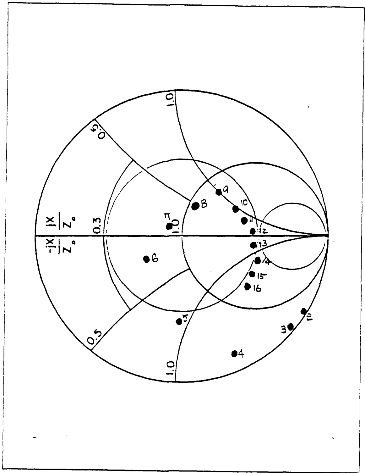
Figure 3.20 Model 3 Impedance Plot in Frequency 2-16 MHz for 4 External Shunt Feeds: Z_0 = 150 Ohm.
