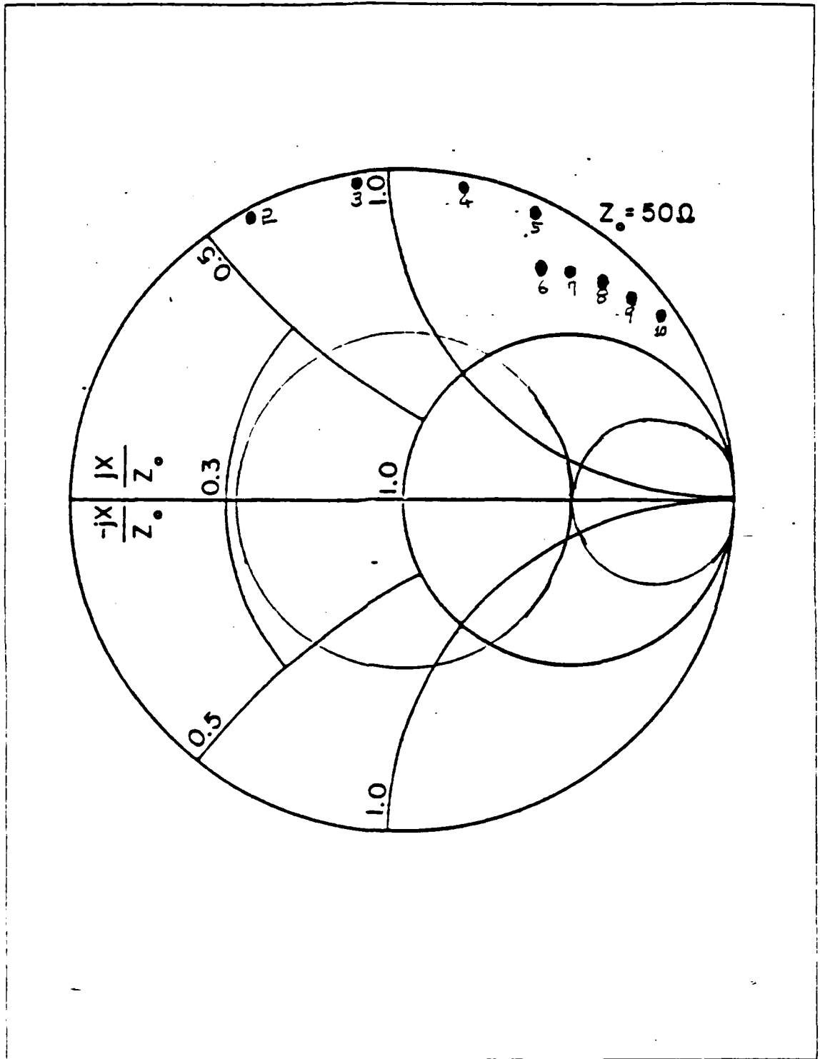
Figure B.15 Model 2 Impedance Plot in Frequency 2-10 MHz for 1 Base Feed: Z_0 = 50 \text{ Ohm} .
