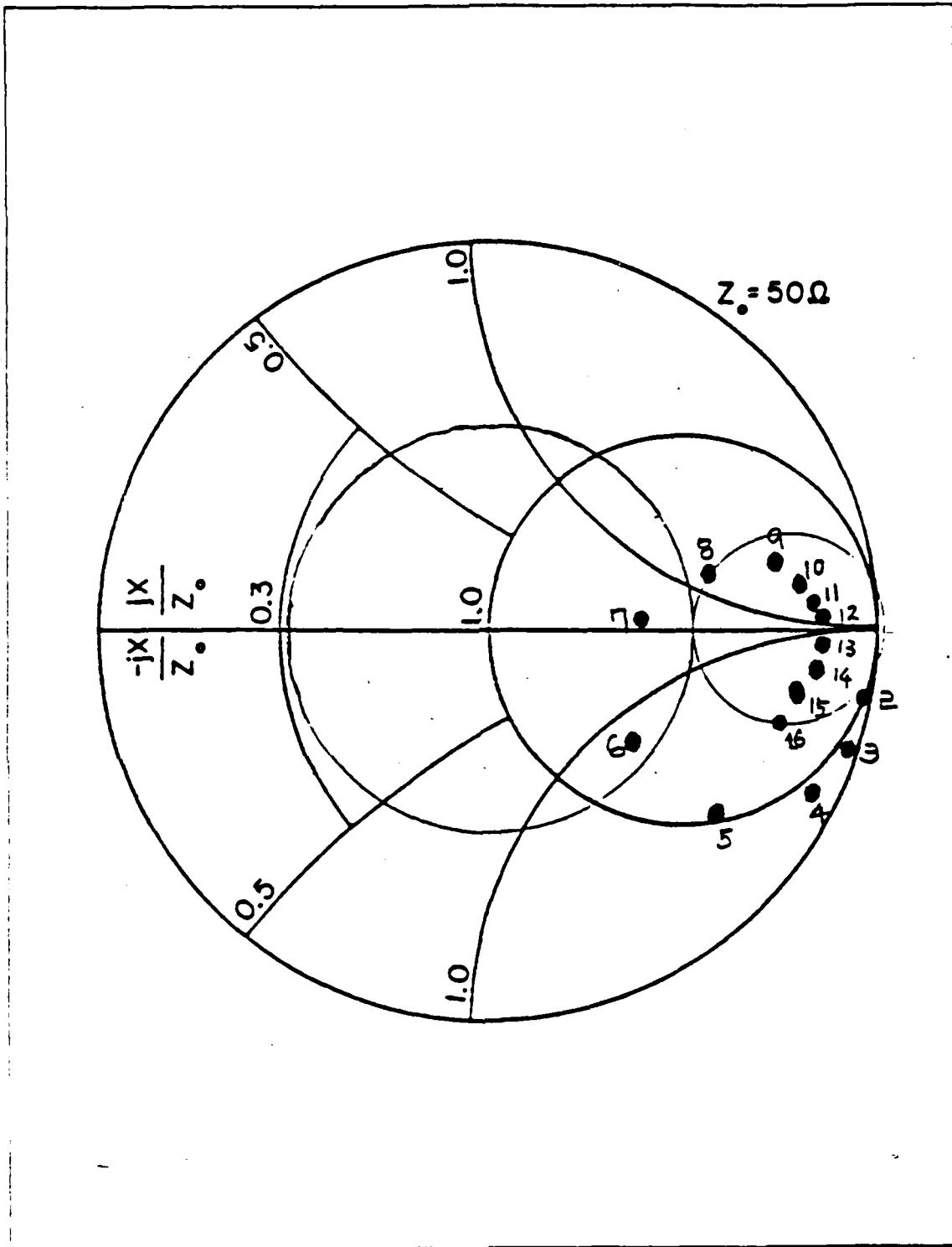
Figure 3.19 Model 3 Impedance Plot in Frequency 2-16 MHz for 4 External Shunt Feeds: Z_0 = 50 \text{ Ohm} .
