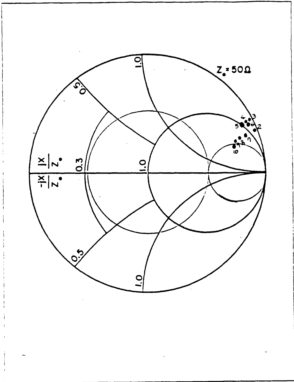
Figure 3.8 Model I Impedance Plot in Frequency 2-10 MHz for 4 External Shunt Feeds: Z_0 = 50 \text{ Ohm} .
