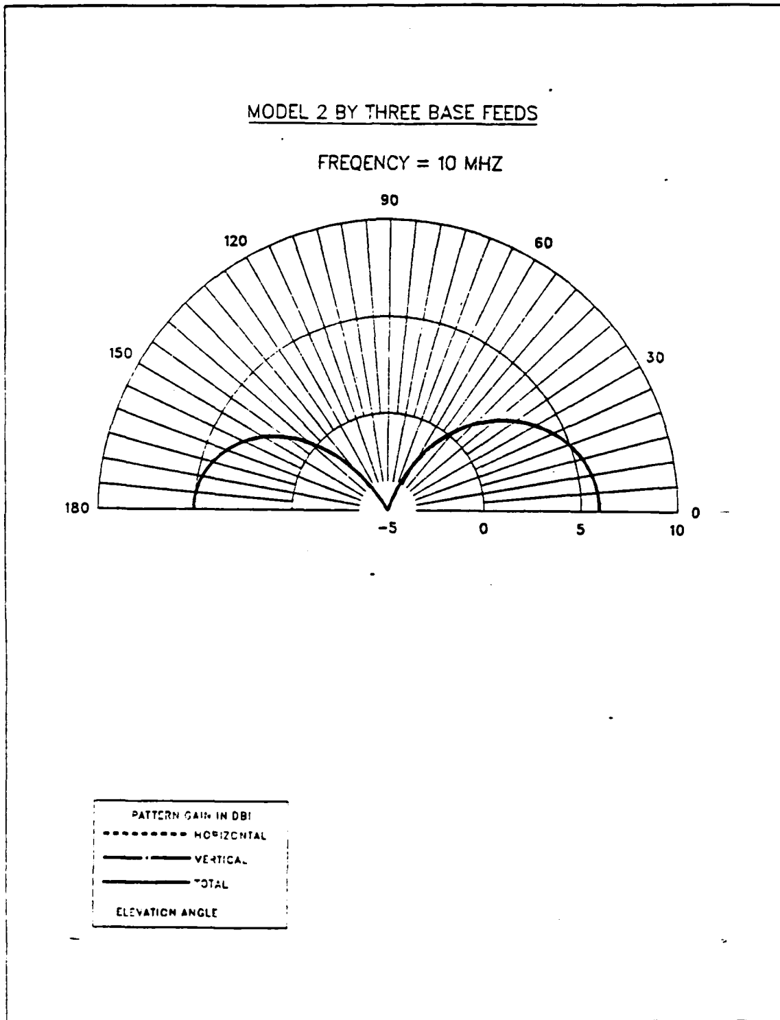
Figure B.6 Model 2 E-Field Elevation Pattern at 10 MHz for 3 Base Feeds.
