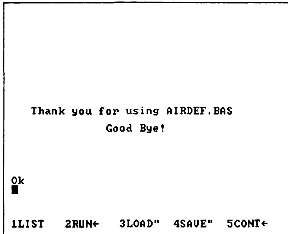
Figure 5. Ending Screen
