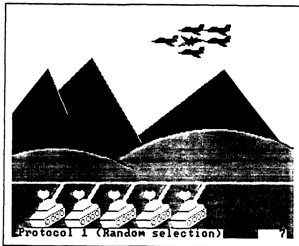
Figure 1. Main Screen
