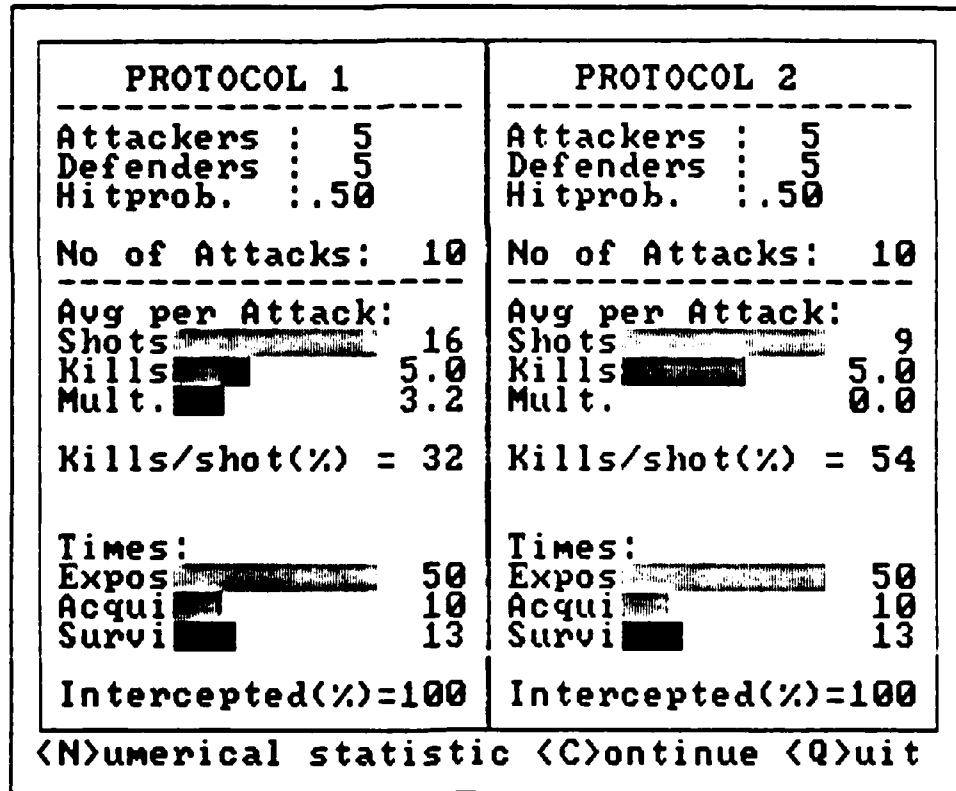
Figure 3. Graphical Statistics
