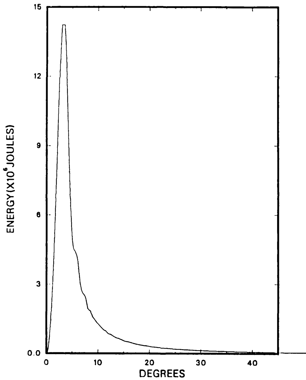
Figure 3.7 Energy per Unit Solid Angle, 10-1000MHz., (Unity Form Factor).
