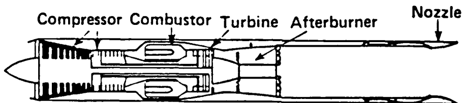
(c) Turbojet
