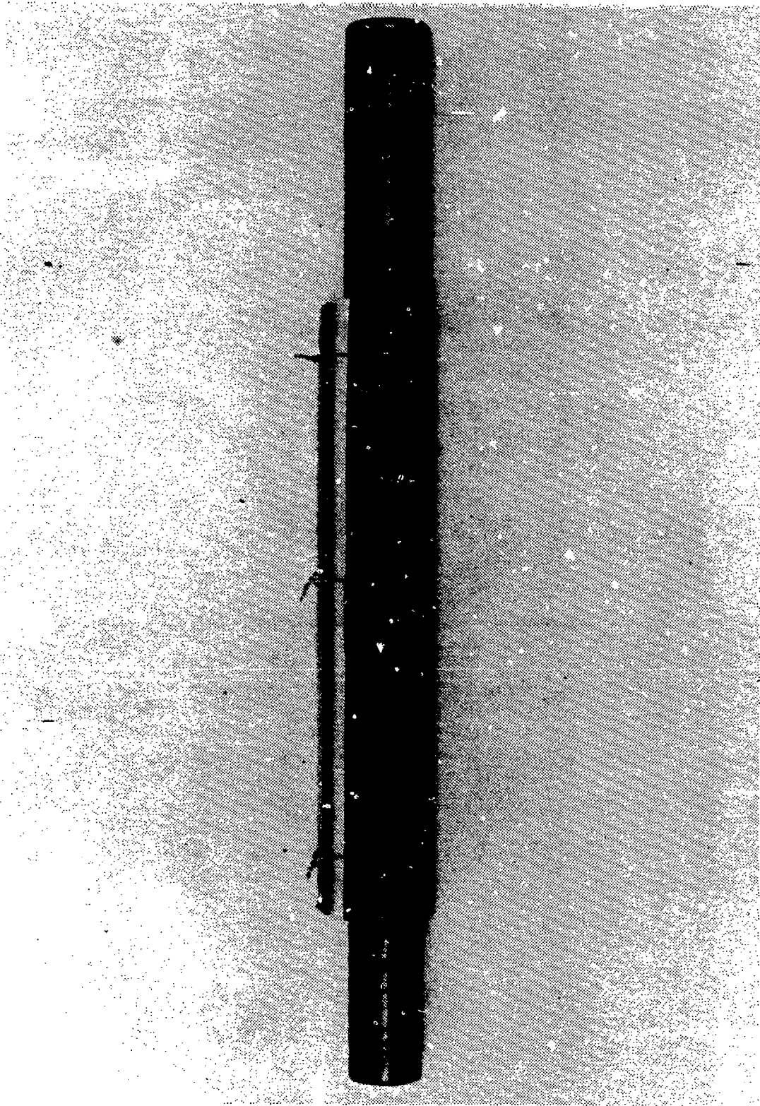
Figure 3.8 A Photograph of Side View of Finned Tube with Fin Tip Insulation Installed.
