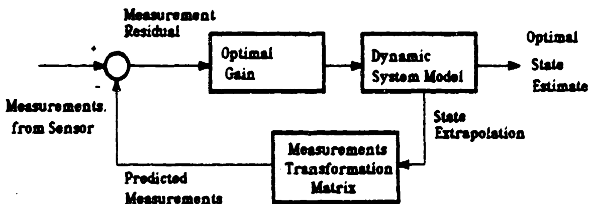
Figure 5.2. Simplified Scheme Of Kalman Filter
