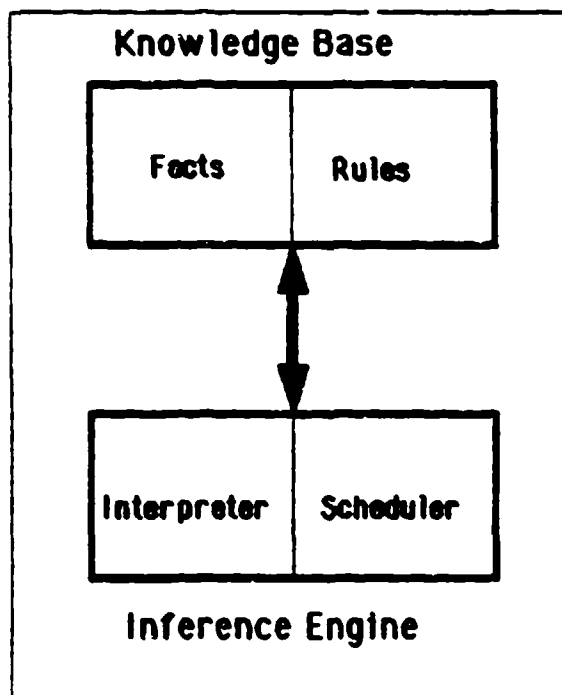
Figure 7.2. Structure of an Expert System
