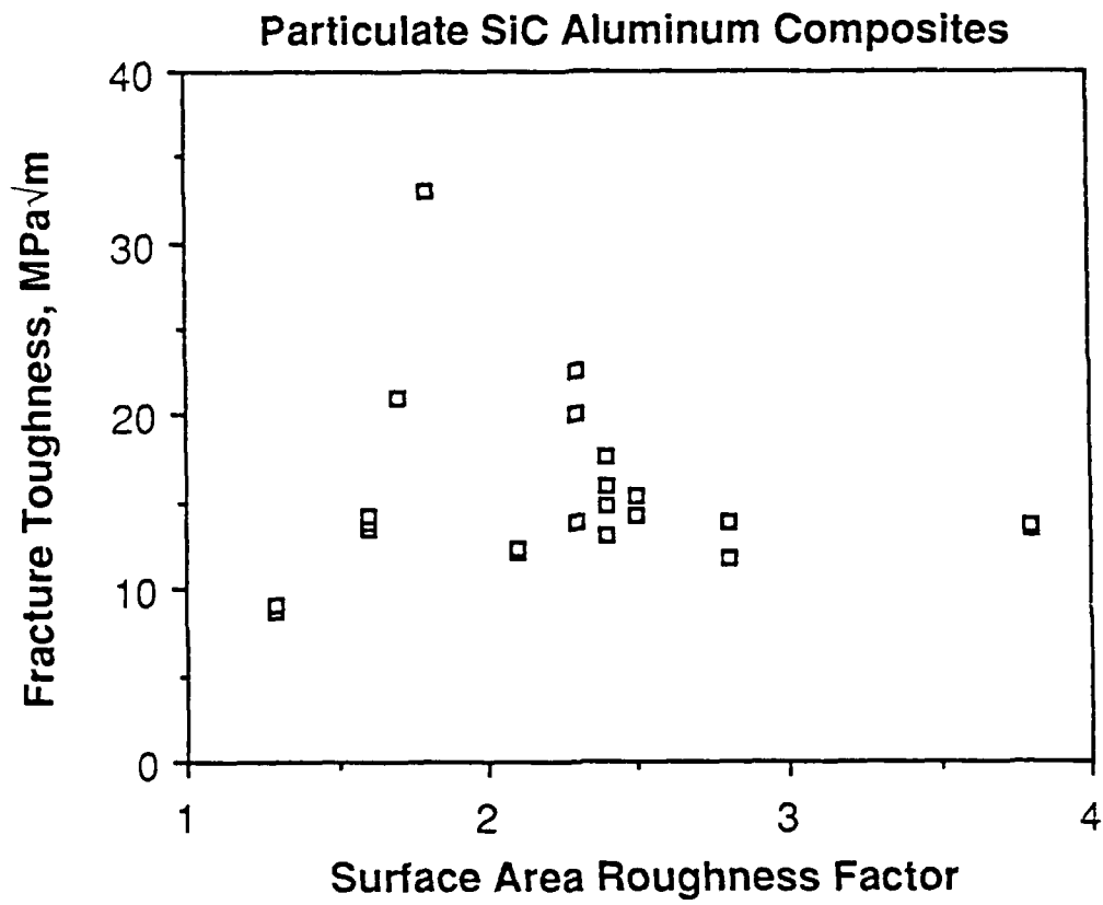
Fig. 5. Comparison of Fracture Toughness and Surface Roughness Ratio for all the composites tested.
