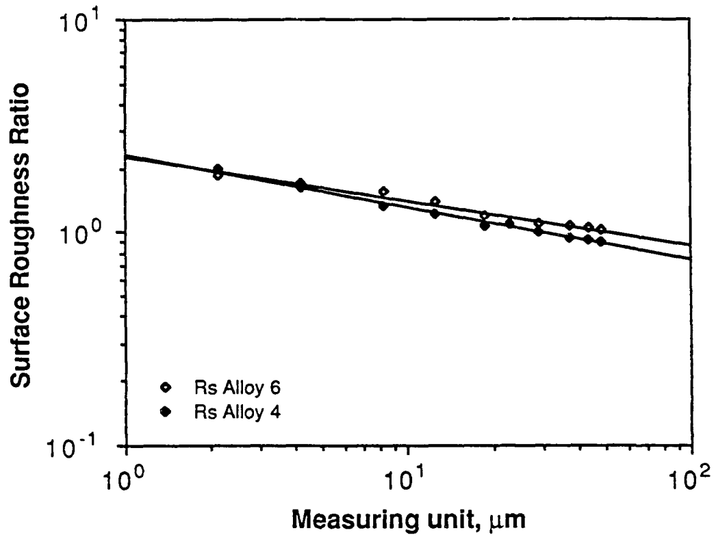
Fig. 3. Surface Roughness Ratio parameters as a function of the measuring unit for two of the composites showing the similarity in magnitude of Rs and the linearity of the relationship when plotted this way.
