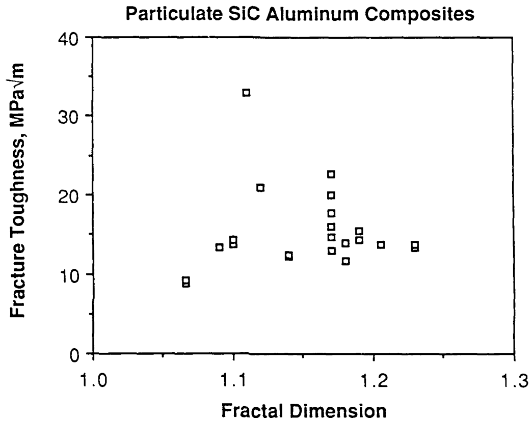
Fig. 6. Comparison of Fracture Toughness and Fractal Dimension derived from the Profile Length Ratio R_L for all the composites tested.
