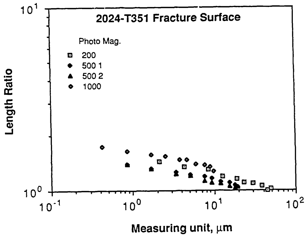
Fig. 4. Comparison of Profile Length Ratio parameters measured at different photographic magnifications.
