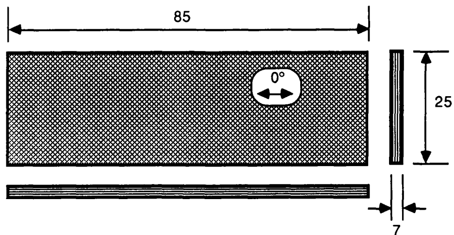
FIG 1b STATIC COMPRESSION TEST COUPONS
