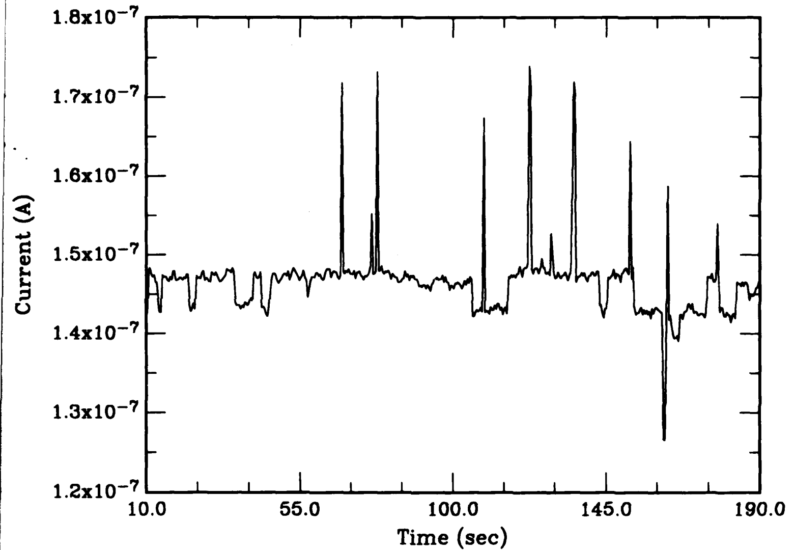
Figure 16. Time-dependent current fluctuations at a fixed bias of 0.875 V of the single quantum dot of the 2 \times 2 pixel dimension (approximately 0.25 \times 0.15 \mu\text{m} ). T = 84 \text{ K} .
