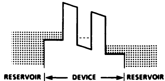
Figure 1. Energy diagram of the resonant-tunneling device model. The device is coupled to electron reservoirs which model the contacts. Shading indicates occupied electron states.
