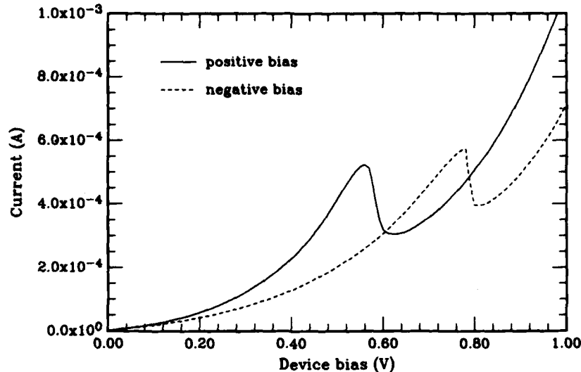
Figure 1. Current - voltage characteristics of a 50 Å GaAs quantum well / 50 Å \text{Al}_{0.35}\text{Ga}_{0.65}\text{As} double barrier heterostructure. The device mesa area =
