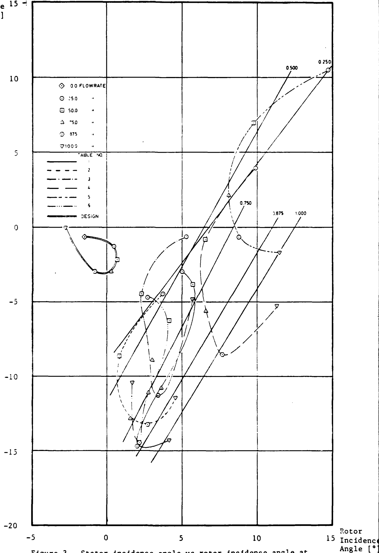
Figure 3. Stator incidence angle vs rotor incidence angle at 60% of design speed.
