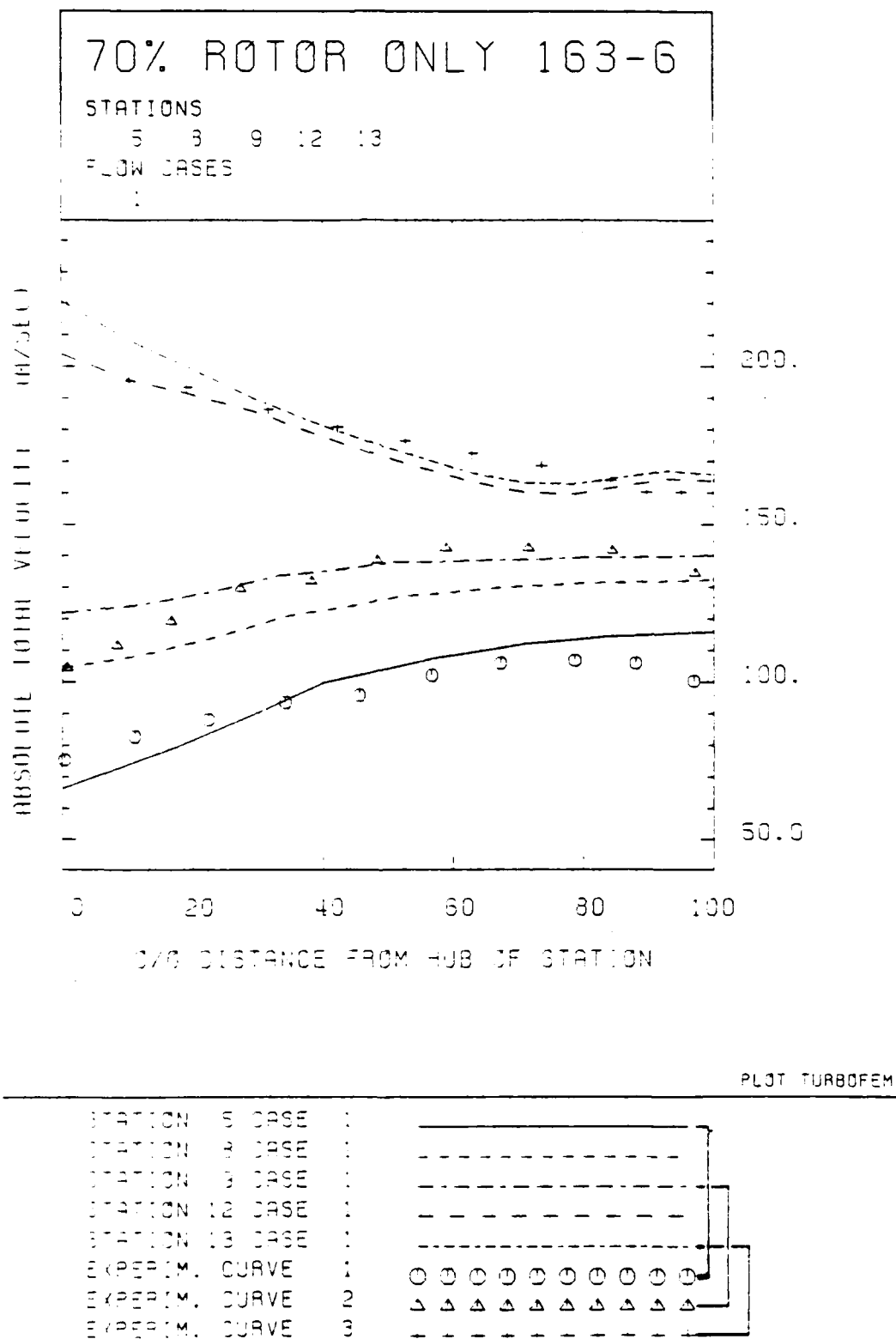
Figure 18. Comparison of measured and calculated absolute total velocity vs blade span at 70% of design speed.
