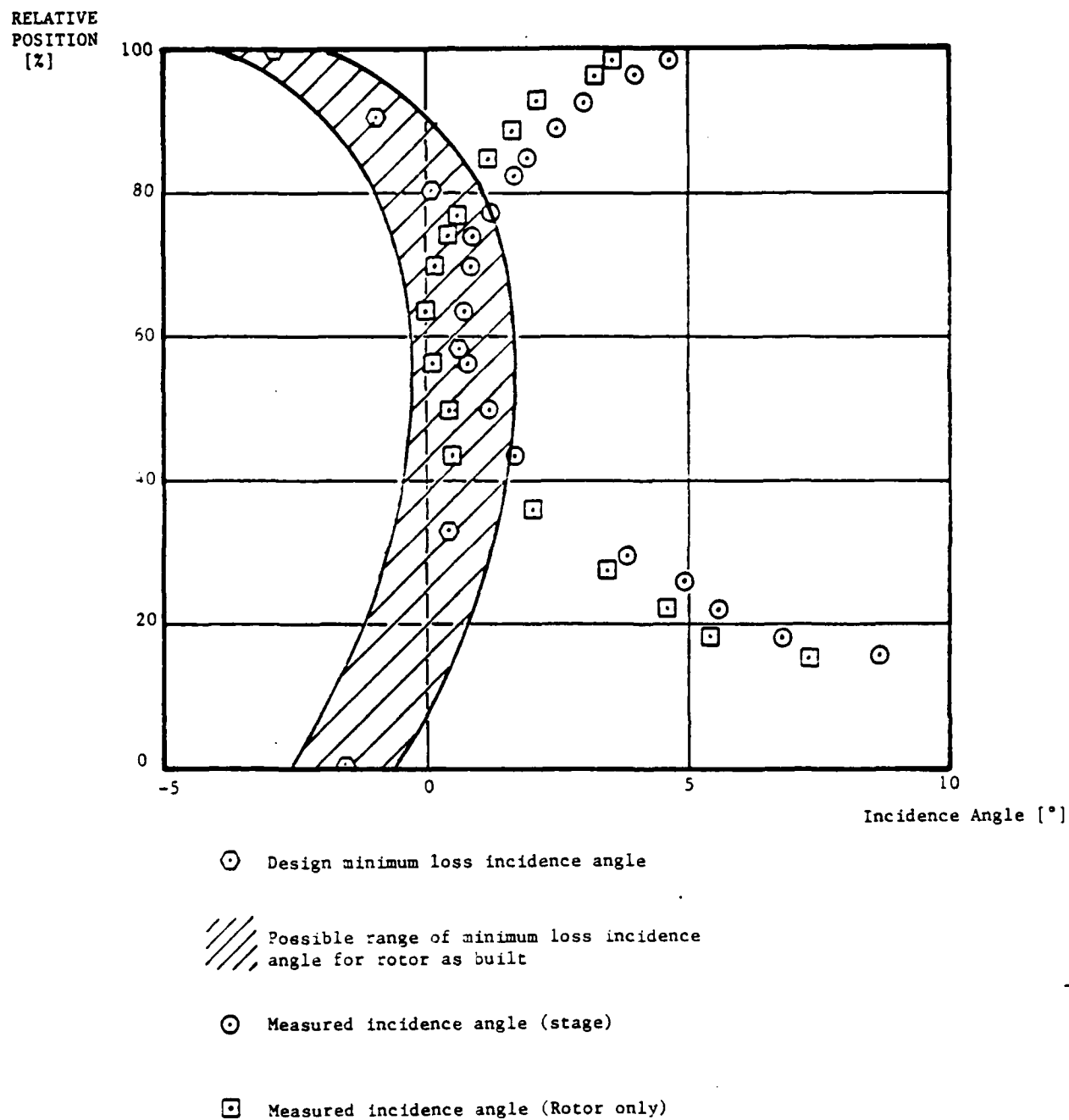
Figure 13. Rotor incidence angle vs blade span for stage and rotor only configuration.
