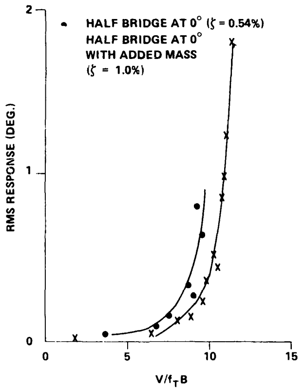
FIG. 5: TORSIONAL INSTABILITY RESPONSE IN SMOOTH FLOW
