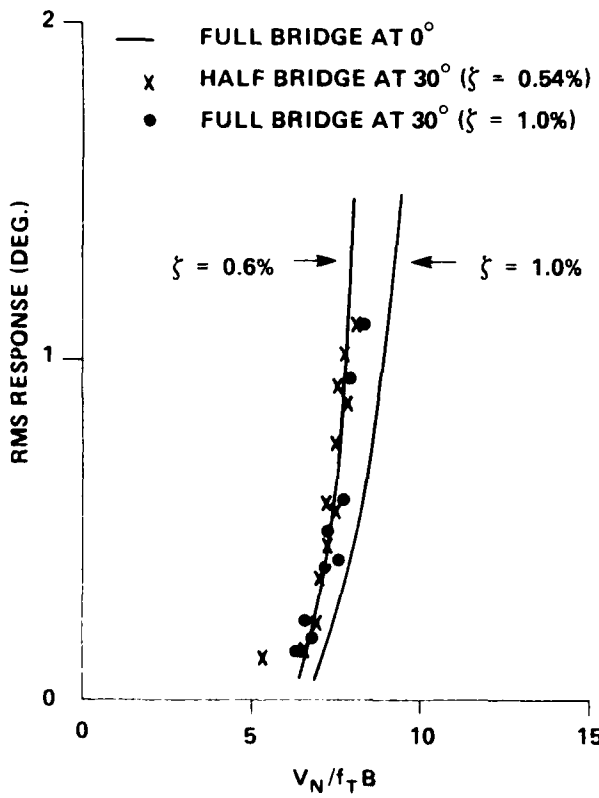
FIG. 5: TORSIONAL INSTABILITY RESPONSE IN SMOOTH FLOW
