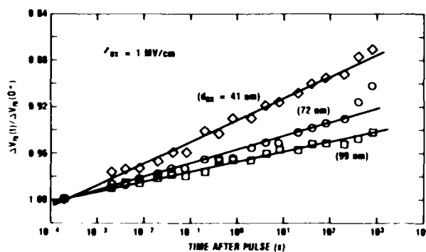
Figure 12. Normalized low-temperature (80 K) flatband voltage recovery data for etched-back oxide samples at 1-MV/cm oxide field, indicating tunneling recombination mechanism for recovery under these conditions.
