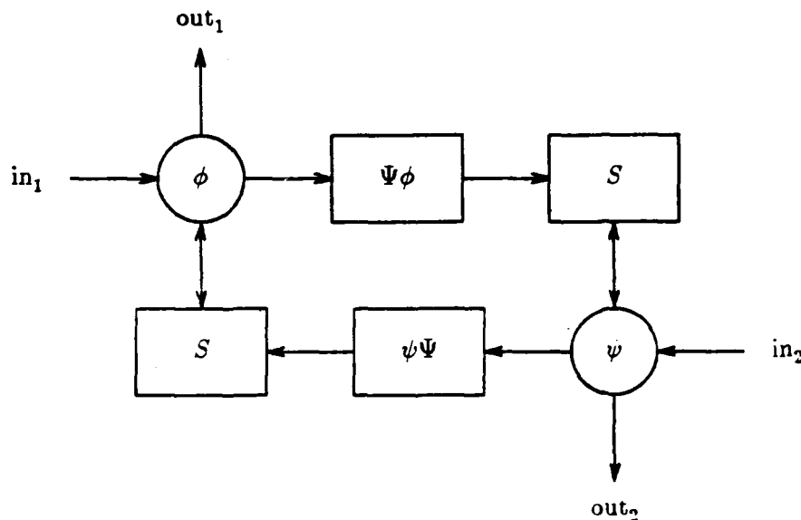
Figure 1. Bidirectional Associative Field Memory
