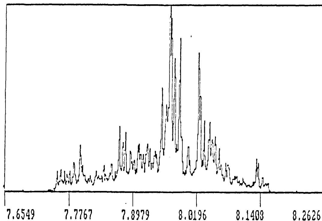
FIGURE 8 Emission from \text{Na}_2(\text{A}^1\Sigma_u^+) excited by a dye laser tuned to the sodium atomic D-line.
