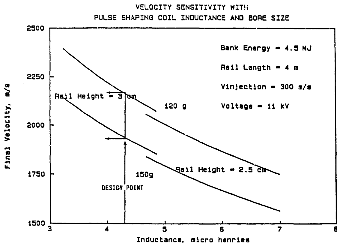
Figure 2.7. Sensitivity of Exit Velocity to Pulse Shaping Coil Inductance, Bore Size, and Projectile Mass
