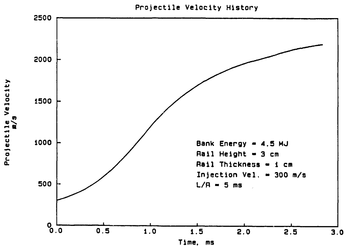
Figure 2.8. Baseline Design Projectile Velocity History
