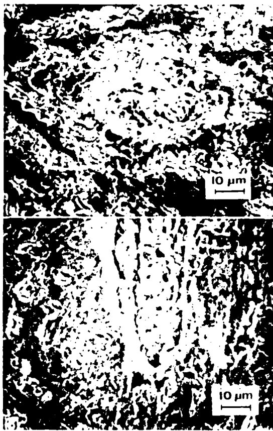
Fig. 5. SEM micrographs of (a) an unimplanted sample and (b) an implanted sample of Stoodly 3 after testing for 20 h. Severe damage occurred to both matrix and carbide phases on the unimplanted sample. Less damage to the matrix phase was observed on the implanted sample.
