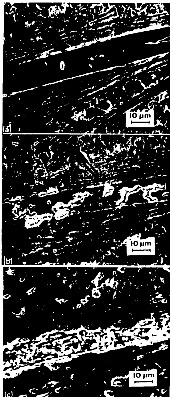
Fig. 4. SEM micrographs of a region on Stoodly 3 titanium-implanted sample 3 after testing for (a) 3 h, (b) 10 h and (c) 20 h.
