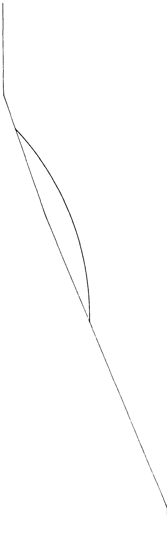
Figure 6.11 - Critical Shear Surface for Pilarcitos Dam Based on a Two-Stage Analysis Employing a Single fc Envelope
