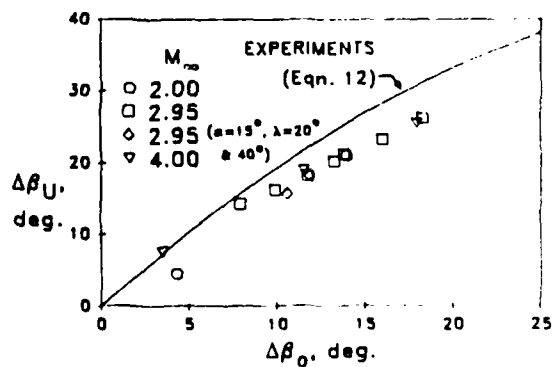
Figure 8: Scaling of computed \Delta\beta_{U1} by \Delta\beta_{O1} .
