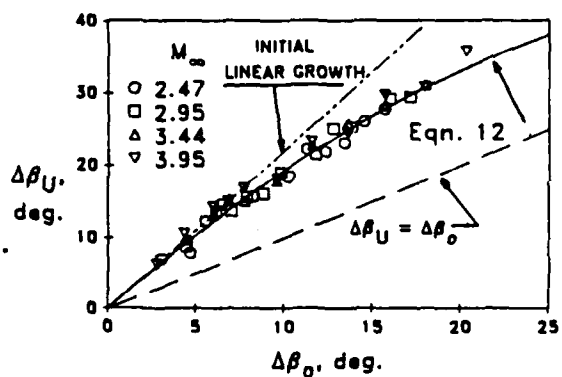
Figure 7: Scaling of \Delta\beta_{U1} by \Delta\beta_{O1} .
