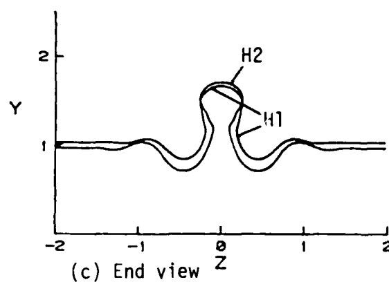
Figure 4.22 - Development of the two hairpin vortices at t=.01 .
