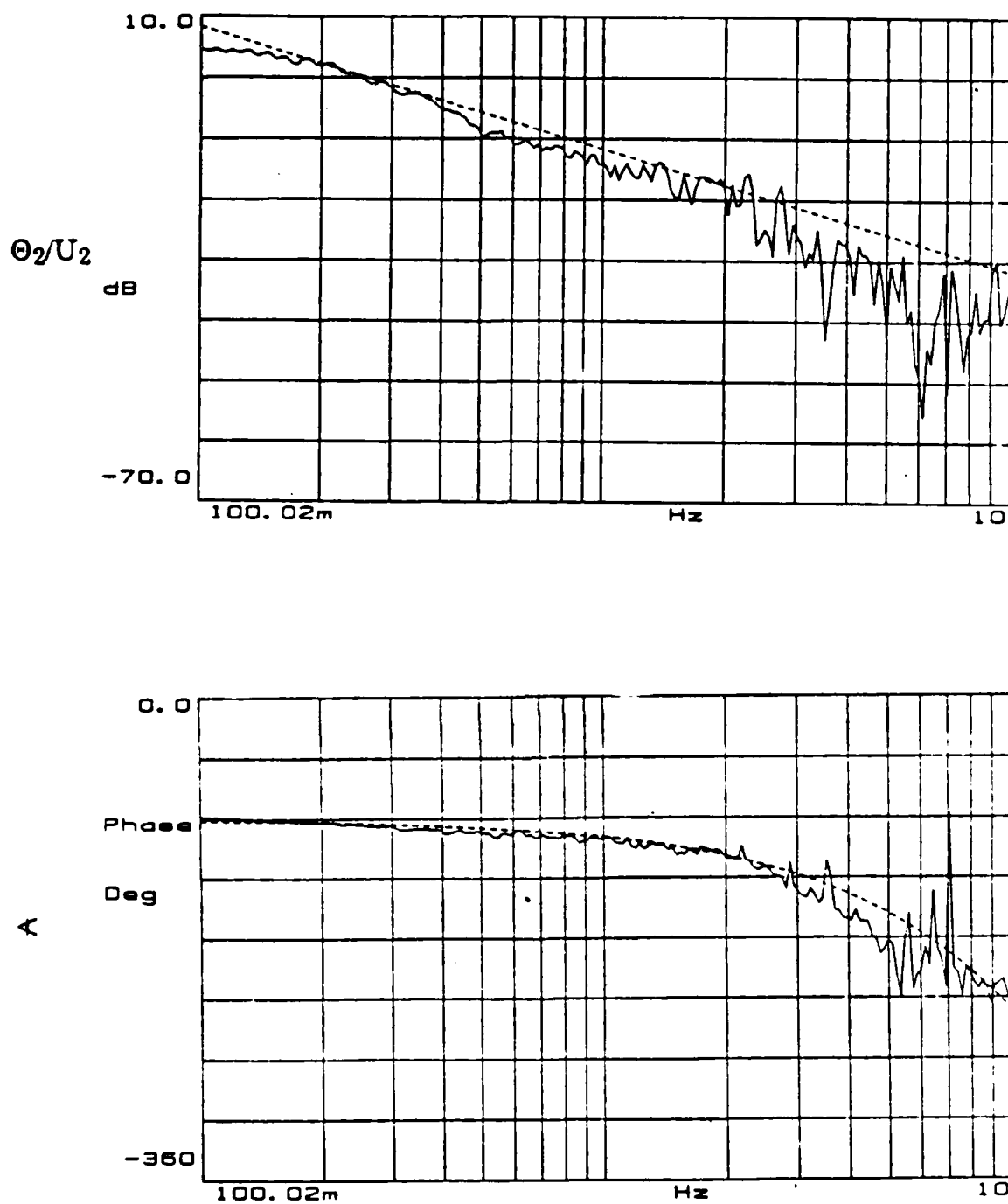
Figure 16 Configuration 1 Linearization - \Theta_2/U_2 data
