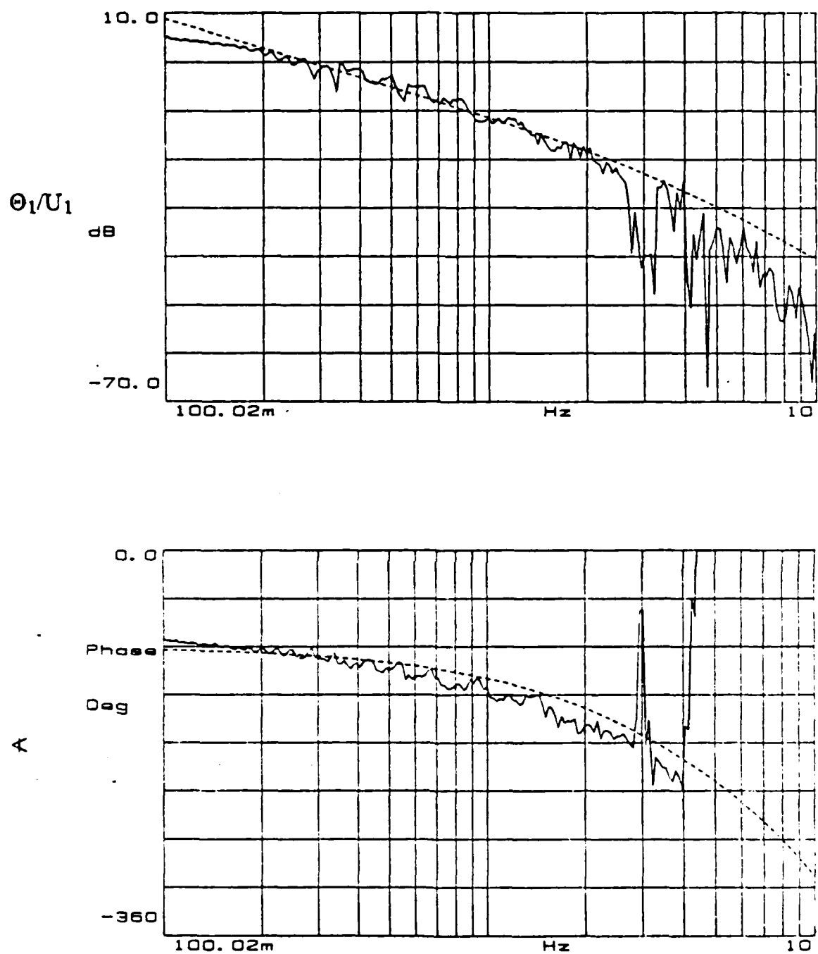
Figure 13 Configuration 1 Linearization - \Theta_1/U_1 data
