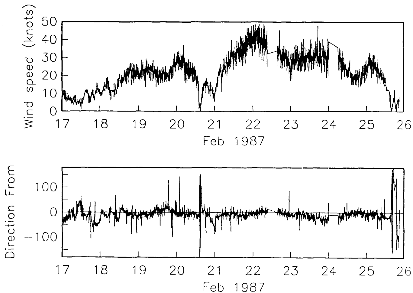
Figure 3. Speed (knots) and direction (degrees clockwise from north) of the wind vectors recorded at two-minute intervals. Note the data gaps on 22 and 24 February.
