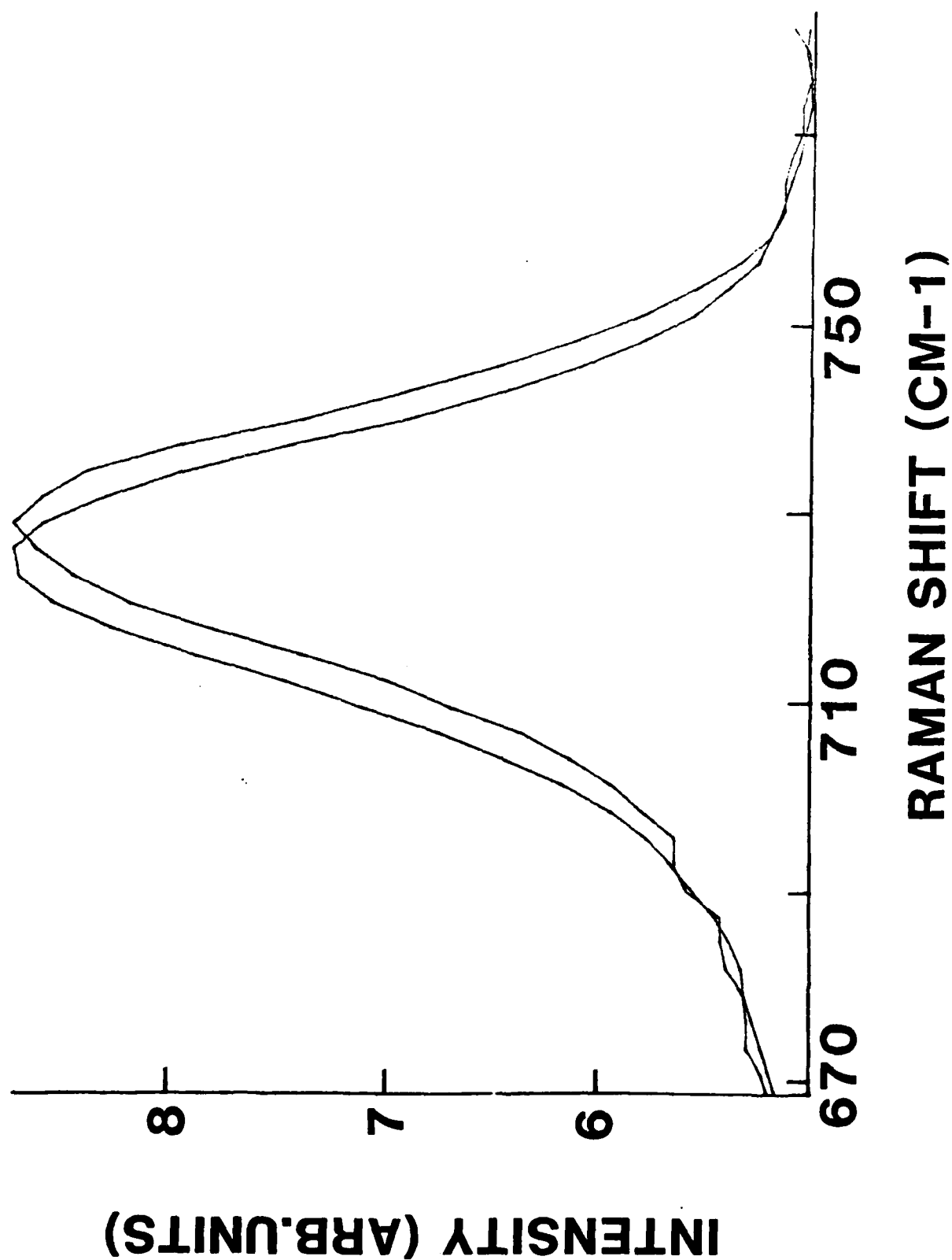
Figure 6. Raman Spectra of the \nu_4 (E') Mode of \text{NO}_3^- Taken for 13 M Aqueous \text{HAN} . The spectrum to the left (lowest frequency peak) is for a temperature of 22^\circ\text{C} ; the other a temperature of -50^\circ\text{C} .
