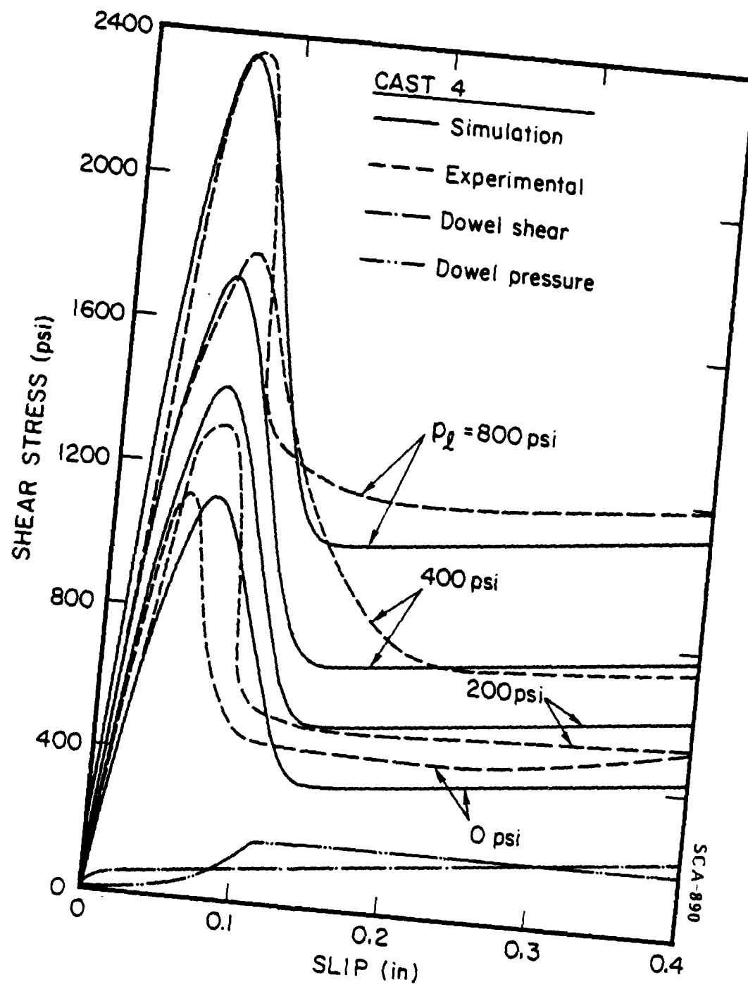
Figure 3.42. Comparison between simulations and Karagozian test results.
