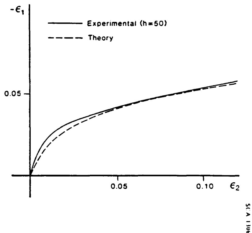
Figure 4.7 Relation between axial and transverse strains under conditions of simple compression.
