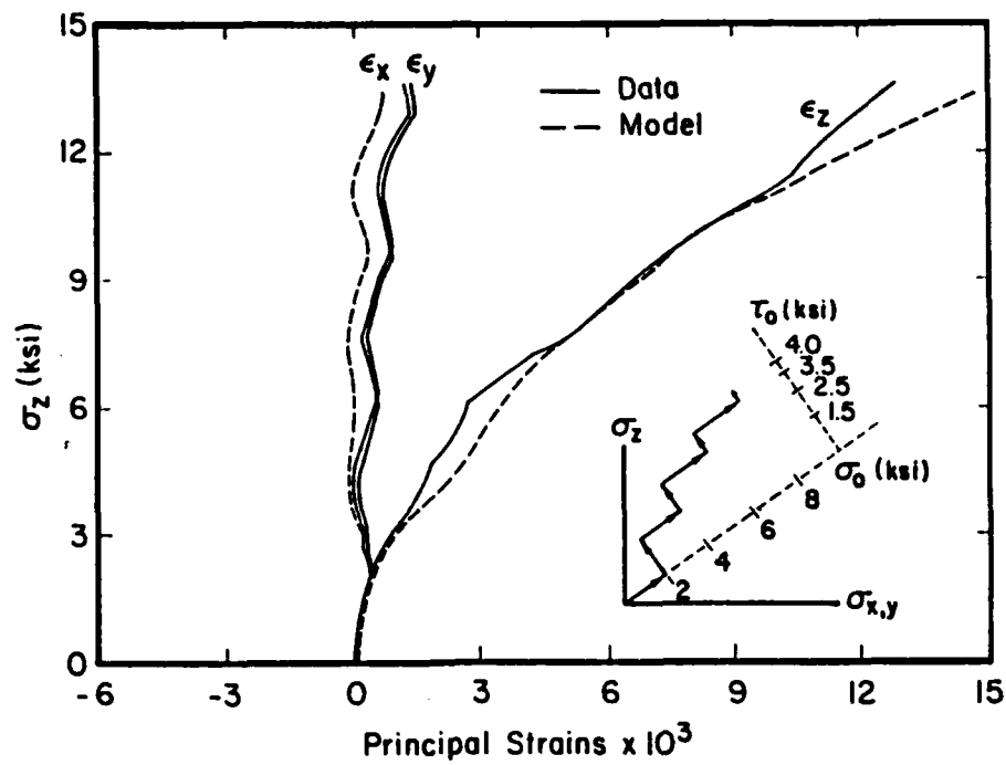
(a) Major principal stress \sigma_z versus principal strains. Insert depicts prescribed stress path.
