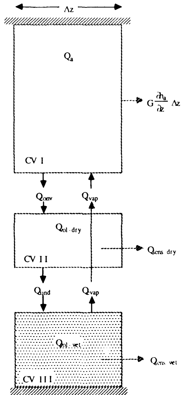
Figure 3-2. Energy balance terms
