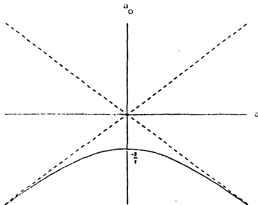
Fig. 1. The stability region lies below the line a_0 + a = 0 , and above the curve a_0 + a = -2a/(e^{ra} - 1) 9
