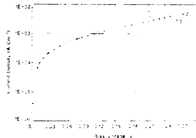
Fig. 8. Fitting of the Simmons model to the low temperature data of Fig. 2. The top material is biased negatively. Parameters used:
