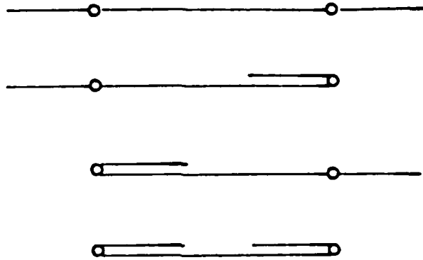
Figure 8 : Fundamental equilibria
