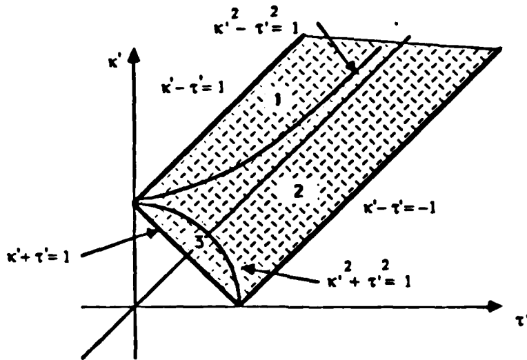
Figure 10 : Parameter-value constraints
