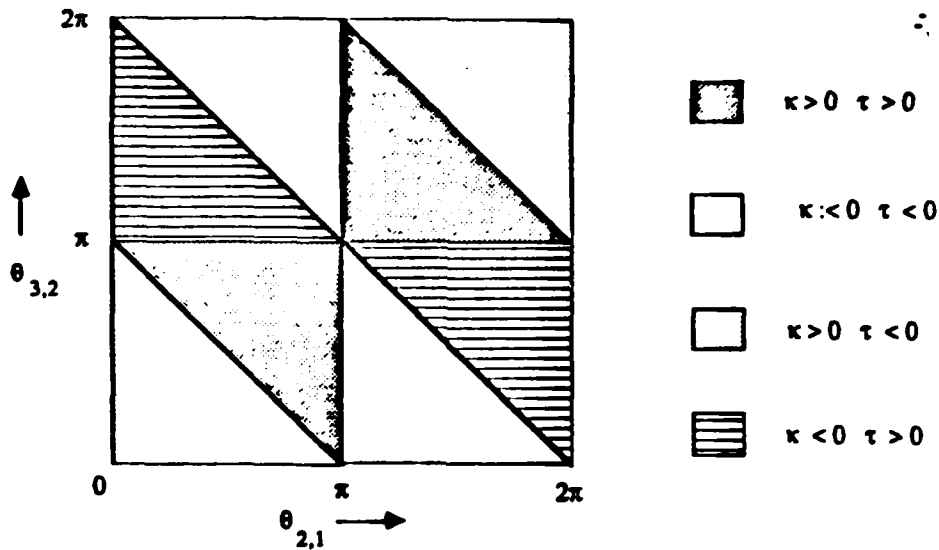
Figure 9 : Parameter-Sign Constraints
