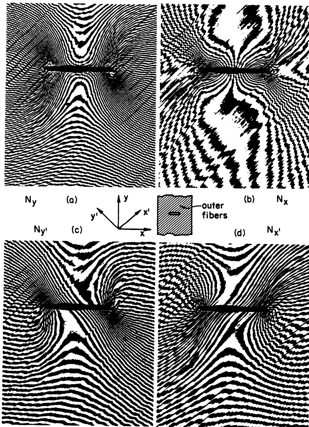
Fig. 6. Displacement fields in a similar specimen, but with stacking sequence [\pm 45/0_2]_s . Sensitivity for \pm 45 deg patterns is \sqrt{2}/f or 0.589 \mu\text{m} per fringe order; for others, sensitivity is 1/f or 0.417 \mu\text{m}/\text{fringe} .
