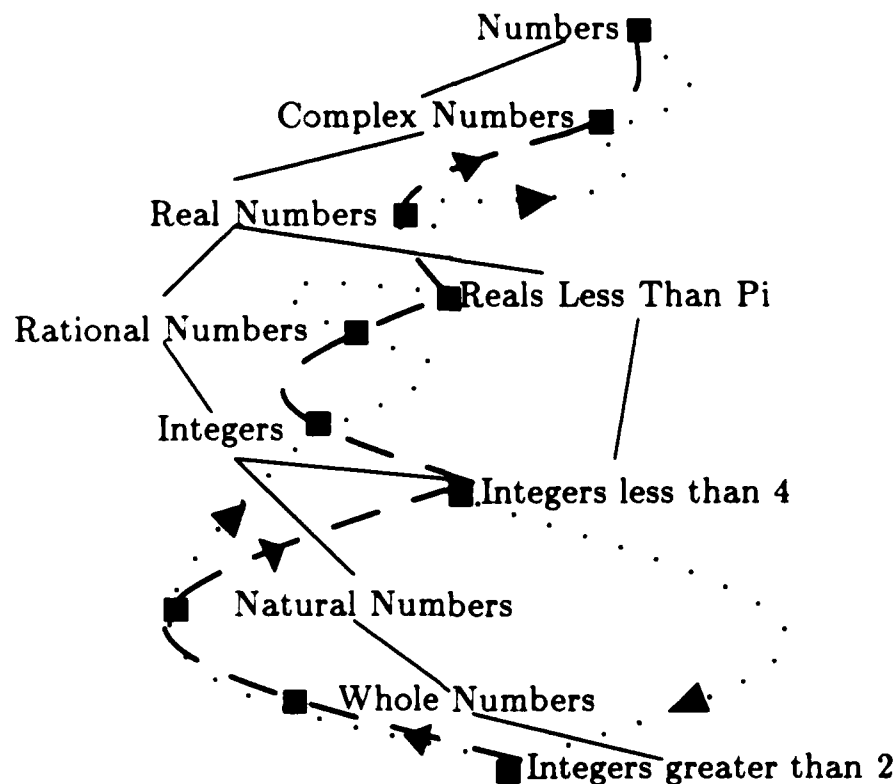
Figure 5-1. When indexing an object, we run the daemons up the lattice in such a way that no type has its daemons run before any of its specializations. This is a potential sublattice of types satisfied by the number '3'; the dashed and dotted lines show two paths indexing might take through the lattice.
