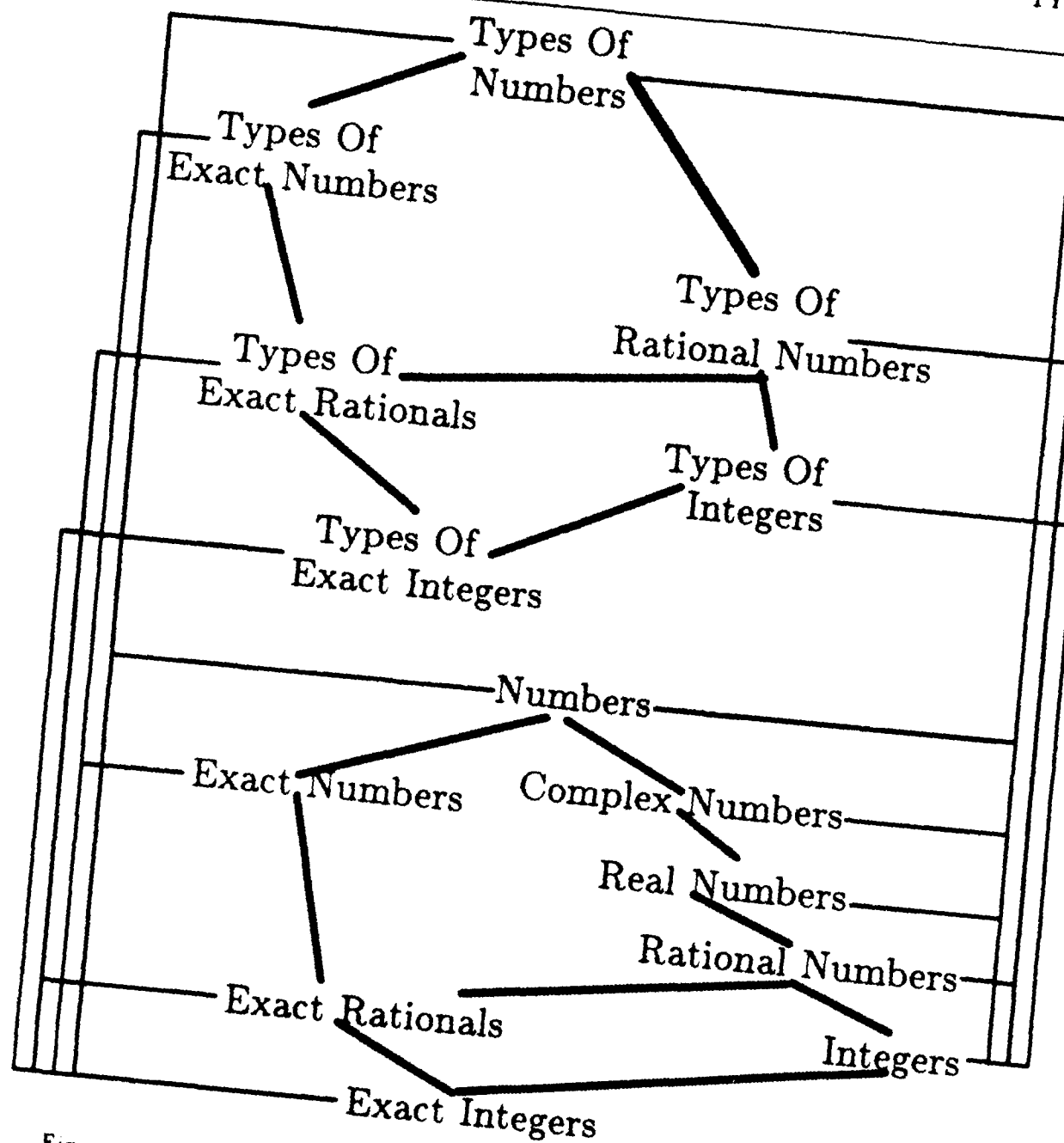
Figure 4-5. The structure around a type is indirectly reflected in the structure around its power set. The bold lines in the figure indicate subsumption in the lattice, while the finer lines indicate satisfaction of types by metatypes.
