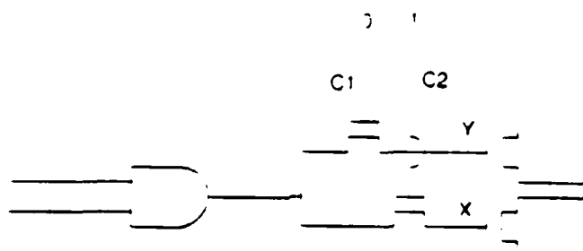
Figure 4.7: Voltage Changes. Under pessimistic enough conditions, asserting C1 can pull X low.
