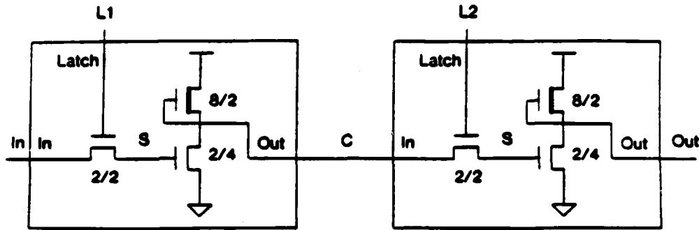
Figure 1.5: Composing Two Latched Inverter Cells to Make a Shift Cell
