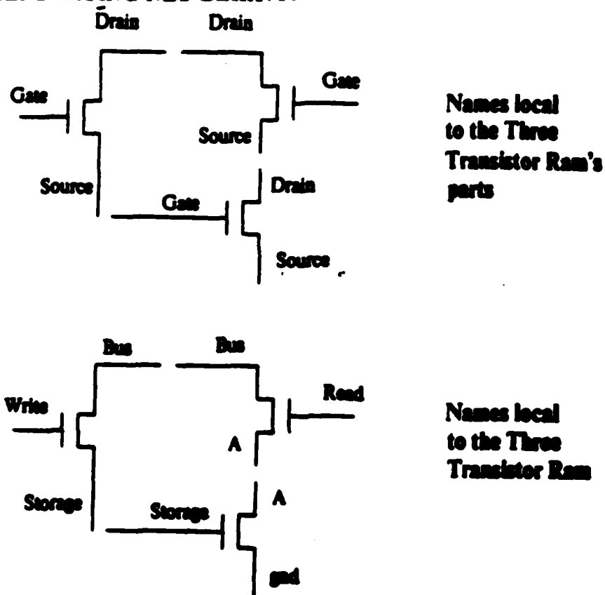
Figure 8.3: Renaming the transistors of the Three Transistor RAM.
