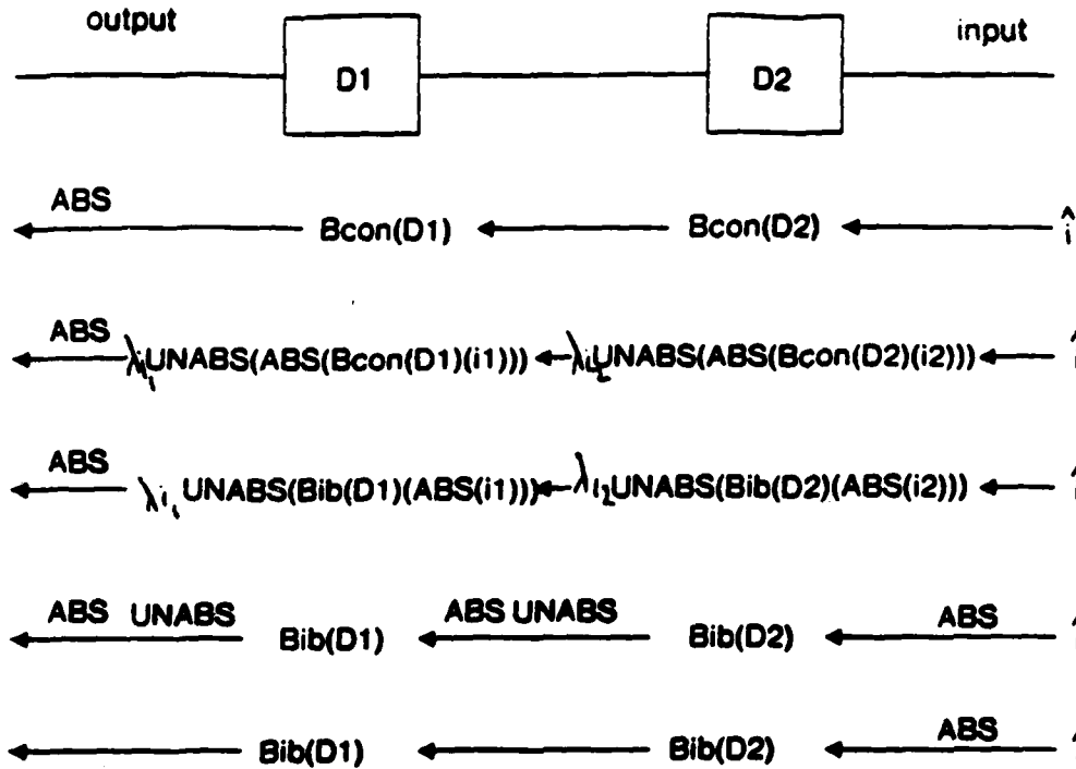
Figure 10.3: Deriving compose_{abs}(B_{IB}(D_1), B_{IB}(D_2))ABS(i) from ABS(compose_{con}(B_S(D_1), B_S(D_2))(i))
