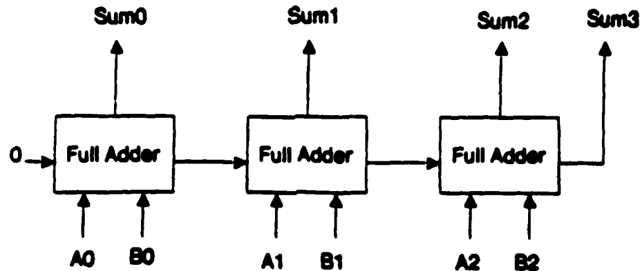
Figure 10.6: 3-Bit Adder
