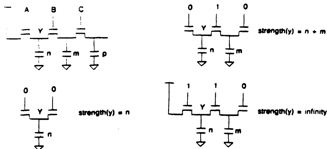
Figure 2.4: Signal Strength
