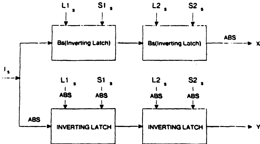
Figure 10.5: The Verification Condition for the Shift Cell. P_{\text{found}} are the constraints derived during verification. INVERTING LATCH represents the intended digital behavior of the Inverting Latch.
