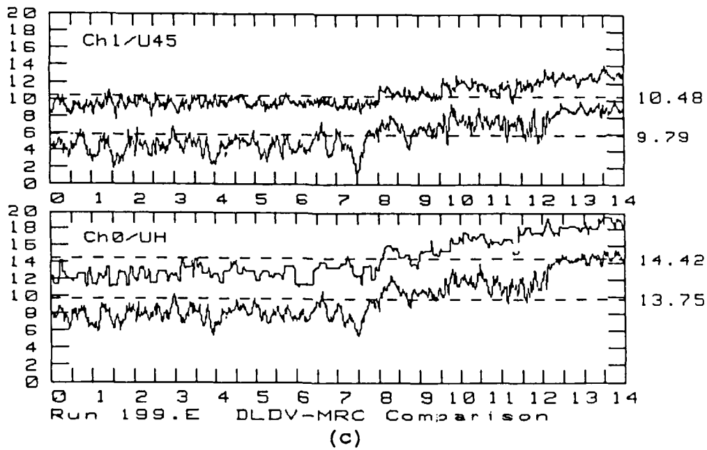
Figure 4. Same as Figure 2, except Run 199.E
