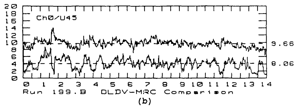
Figure 10. Same as Figure 9, except Run 199.B.
