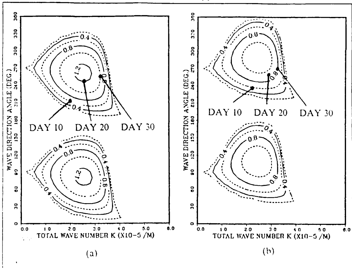
Figure 3.7 Growth Rate Positions of Model Output Waves for Shear Velocity of 0.4 m/s.
