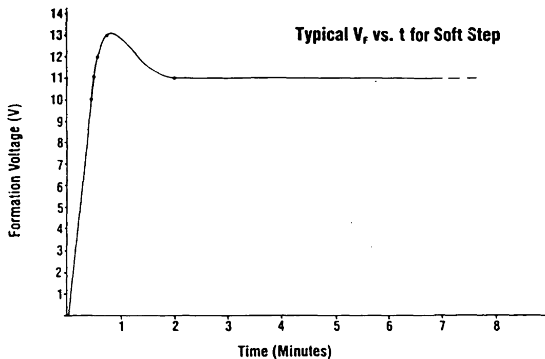
Figure 18 Typical forming voltage characteristic for the porous anodization. Nine minutes of anodization with a constant current density of about 1.5 \text{ mA/cm}^2 at 6^\circ \text{ centigrade} in the sulfuric acid electrolyte produced a 6000 \text{ \AA} thick oxide.
