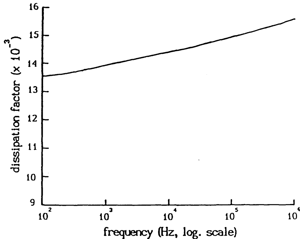
Figure 17 Variation of the dissipation factor with frequency for a hard oxide film of alumina anodized with a 100 V forming voltage. 5
