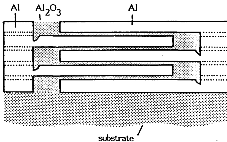
Figure 56 Cross sectional view of proposed method to create comb structure via photo resist masking. Note that the thickness of the successive layers is staggered.
