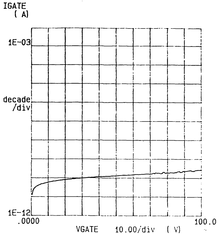
Figure 37b Same as for Figure 37a but this plot represents the third pass or ramping up of the voltage. Notice that the capacitor has been 'healed' from most of its small defects up to 100V. The following resistivities were obtained for this 41\text{cm}^2 , 8000\text{\AA} thick capacitor structure:
