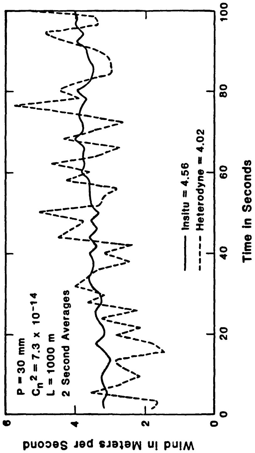
Figure 6 - Wind Measurement, Target at 1000 Meters, Z Log Ratio Processed
