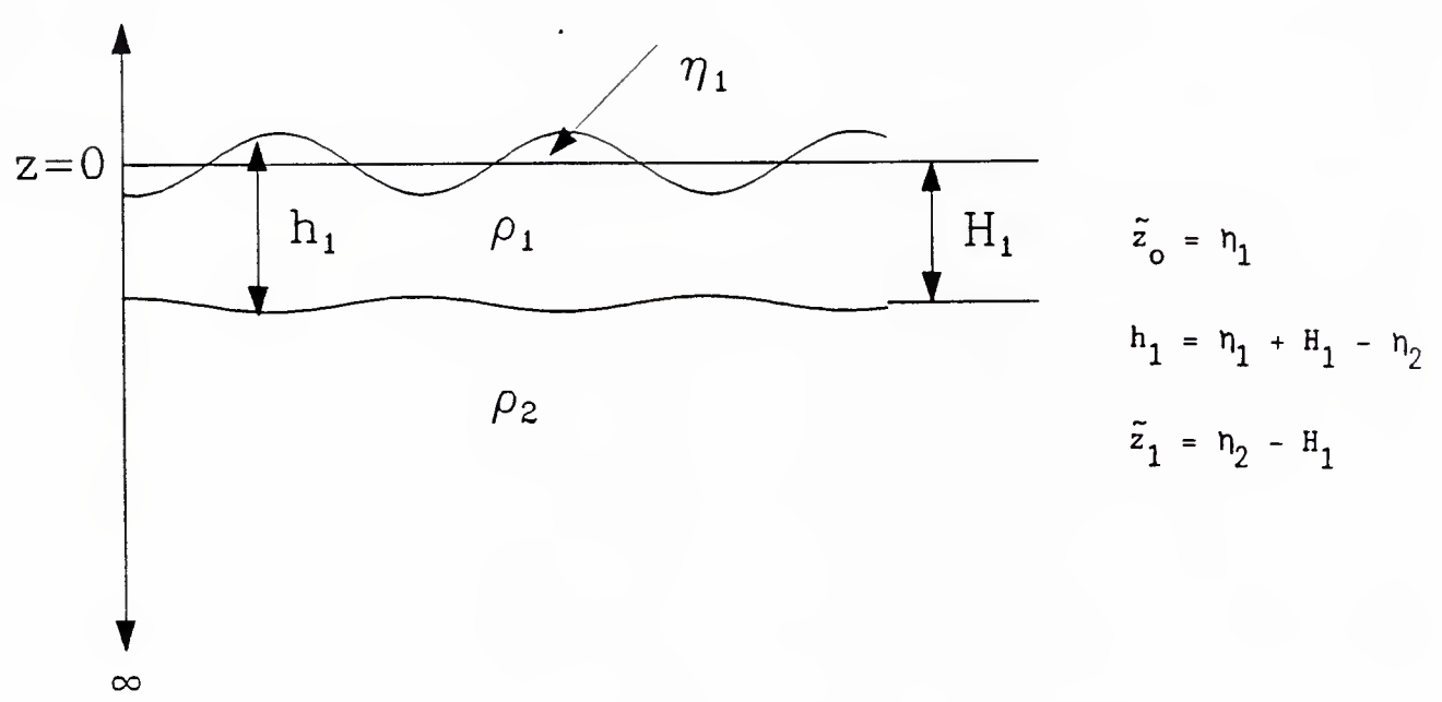
Figure 13. A vertical cross section of a one active layer, reduced-gravity model.
