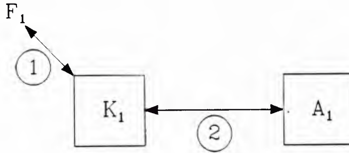
Figure 8. Energy transfers in a one-layer, finite depth model for the layer-layer formulation.
