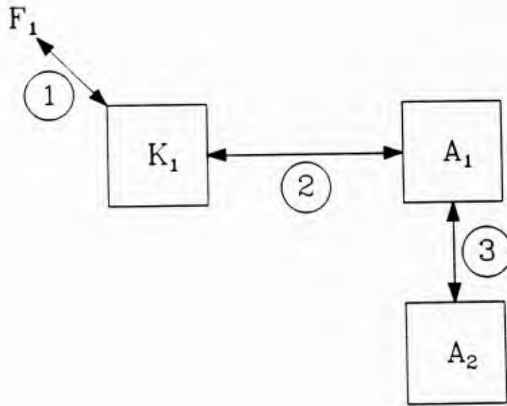
Figure 14. Energy transfers in a one active layer, reduced-gravity model for the layer-layer formulation.
