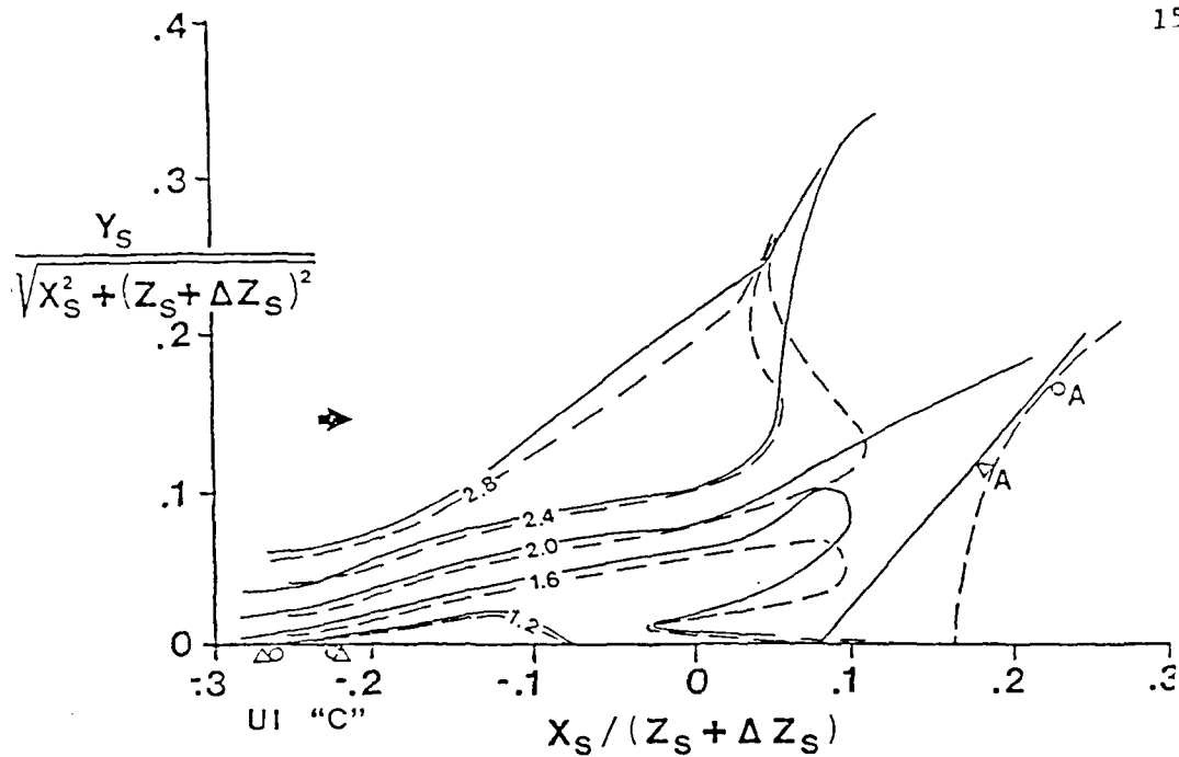
Figure 6a: \alpha = 30^\circ , \lambda = 60^\circ Swept corner (solid) and 25^\circ semicone (dashed) Mach contours.
