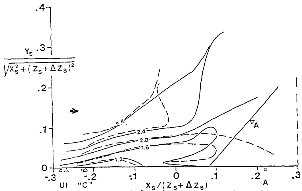
Figure 6b: \alpha = 30^\circ , \lambda = 60^\circ Swept corner (solid) and 17.5^\circ fin (dashed) Mach contours.
