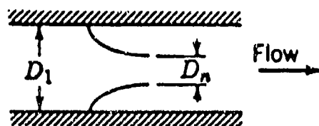
FIGURE 13. Steady Flow Characteristics For a Long Radius Flow Nozzle (Ref. 4, p. 431)
