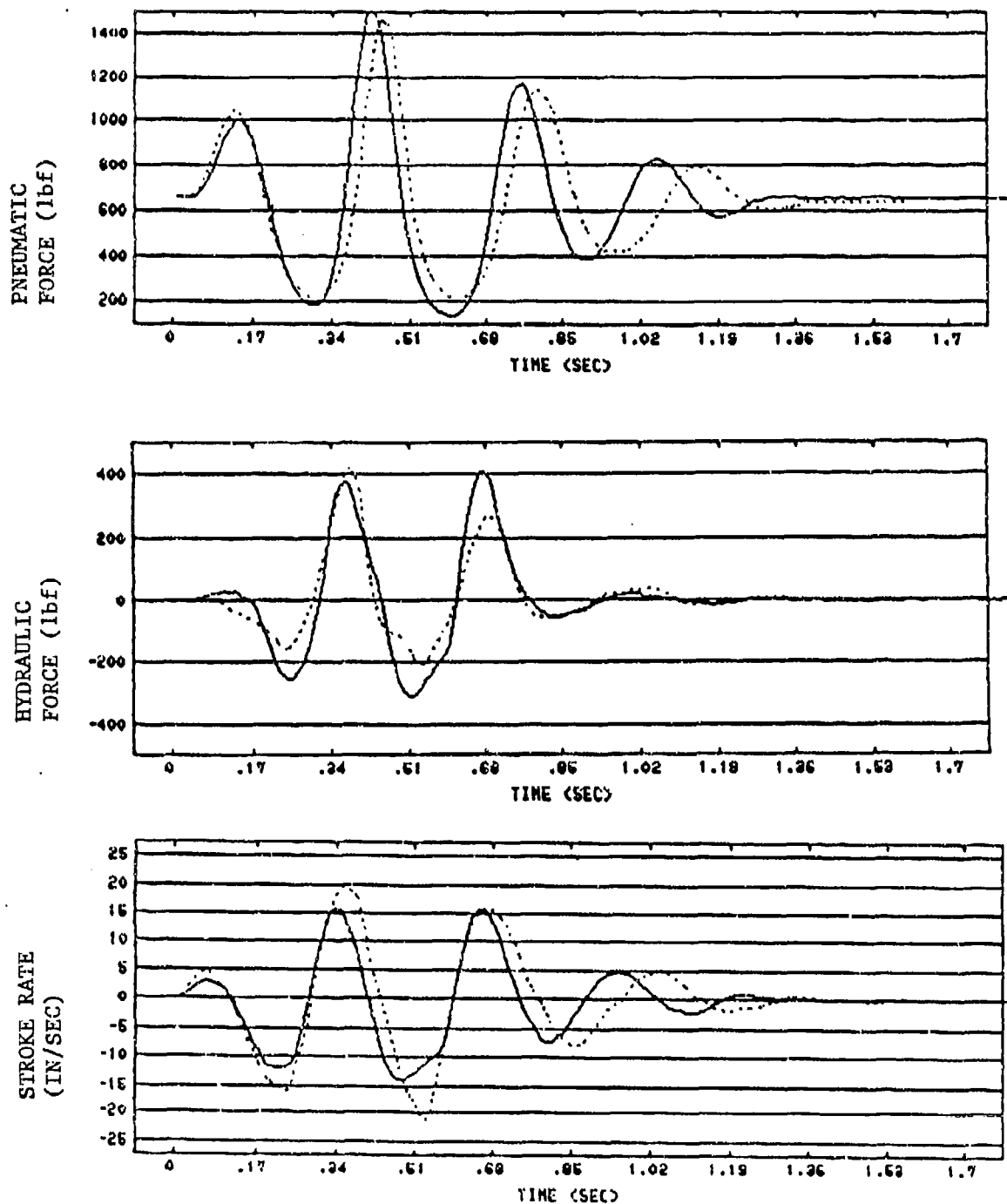
TAXI SPEED LEGEND FIGURE 50. Model Gear (Phase 11a) 5.7 Ft/s _____ vs. A-37 NLG (Phase 1) 10.0 Ft/s .....
