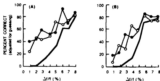
Fig. 4. Effect of adding error from a depth estimate to the psychometric function obtained in the standard frequency-discrimination experiments. An estimate of the psychometric function resulting from adding a depth judgment to the spatial-frequency-discrimination process is shown (bold lines). The probability-density function of depth error is Gaussian with \sigma = 3\% (see the text). Results of standard frequency-discrimination experiments (filled symbols) and object-frequency discrimination experiments (open symbols) are also shown. Observers were JDC (A) and CAB (B).
