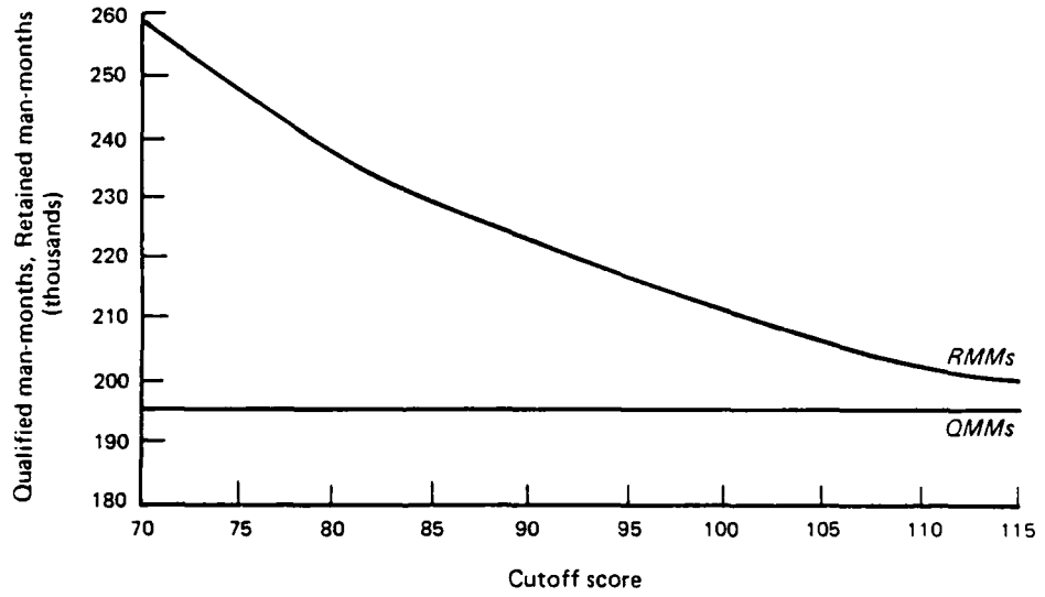
FIG. 7: ILLUSTRATION OF MAJOR VARIABLES: RAND 2
