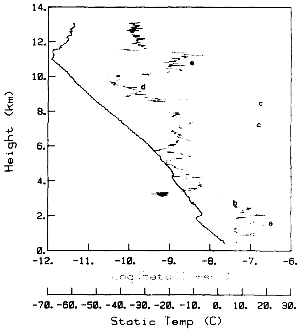
Figure 25A. Climb out of Bodo, 13 March 1986. Observer's log: a - weather hazy; b - top of haze at ~ 2.3 km; c - in slight haze and some cirrus cloud (data shows signal saturation); d - above all haze; e - no visible cloud or haze, very strong signals.
