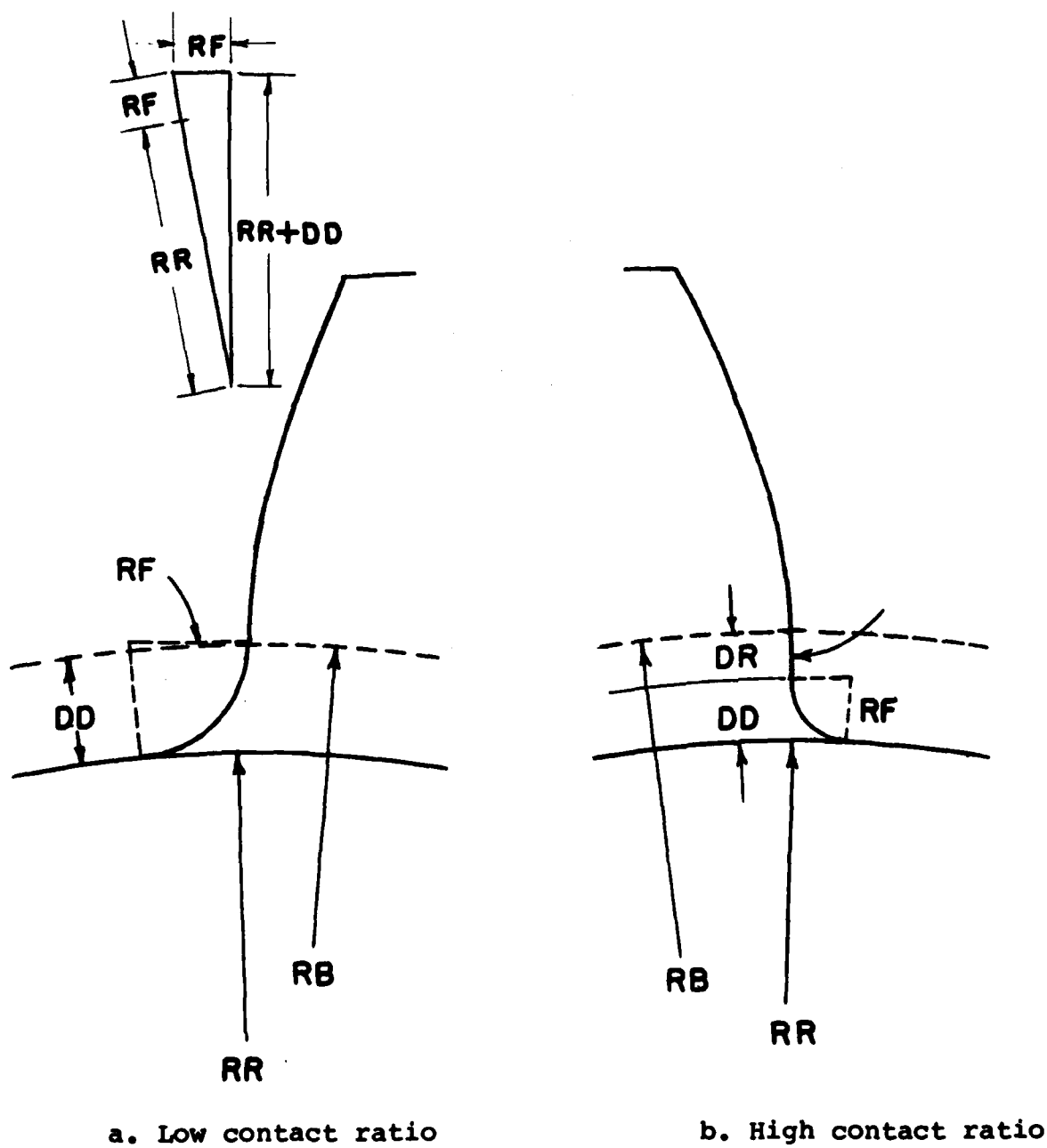
Figure 2-9: Fillet geometry
