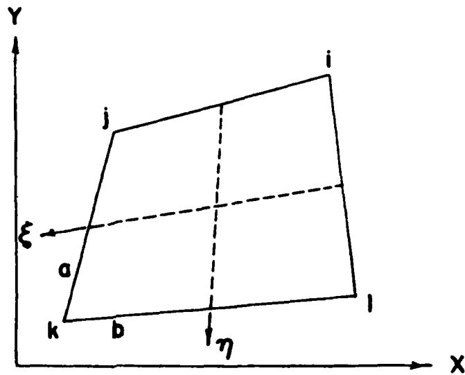
(a) General linear quadrilateral element
