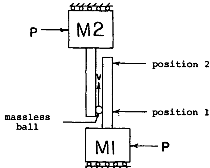
Figure 5-1: Meshing cantilever beams
