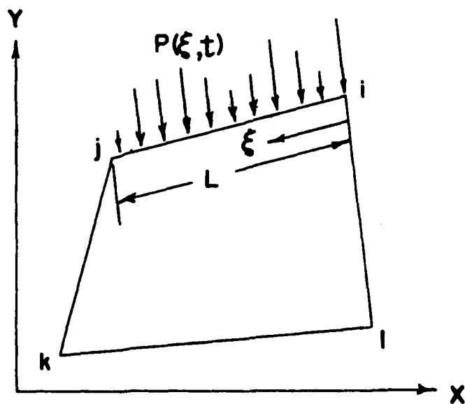
(b) Generalized force application
