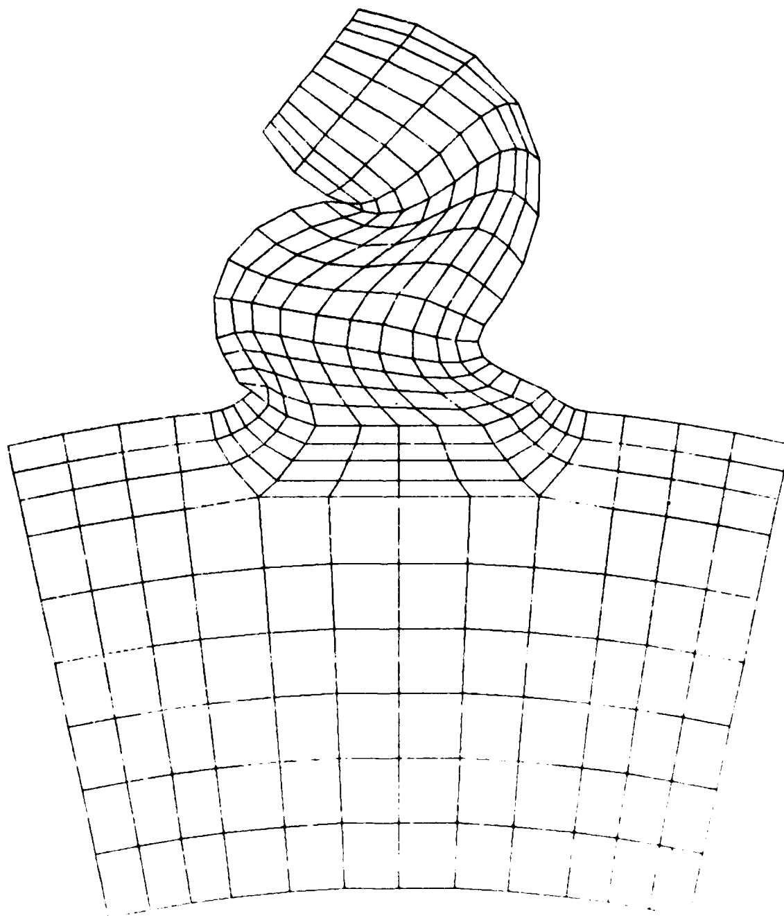
Figure A3-14
