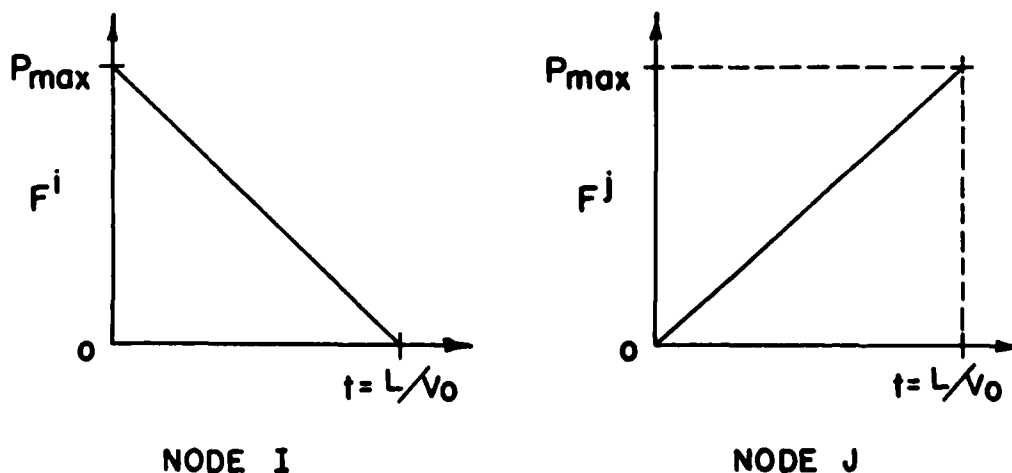
Figure 2-18: Linear force histories
