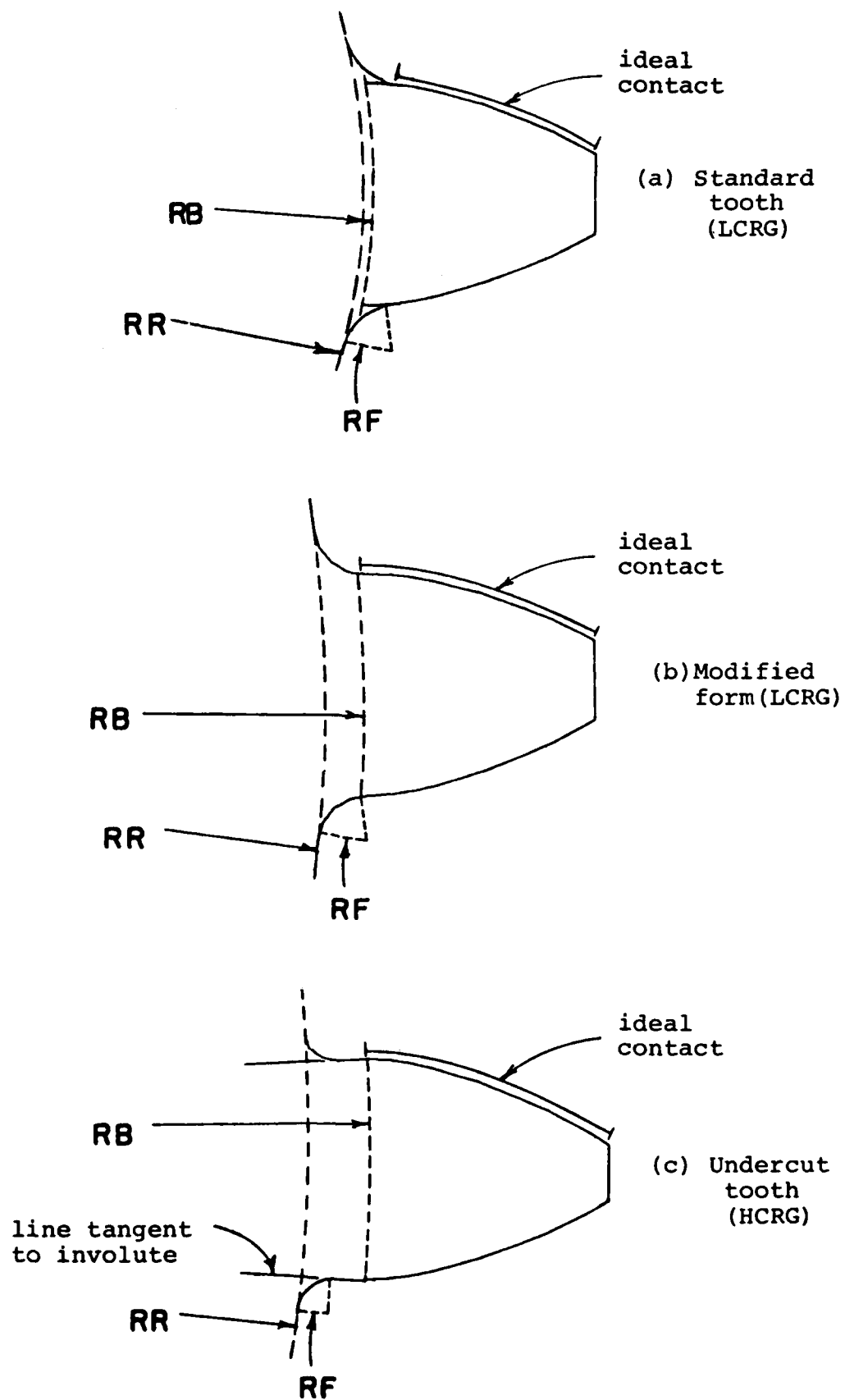
Figure 2-8: Fillet radius geometries
