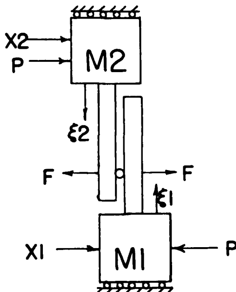
Figure 5-2: System parameters
