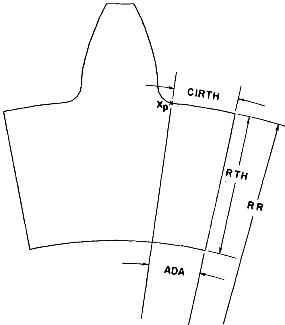
Figure 2-11: Completed profile and rim geometry
