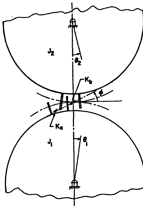
Figure 1-2: Dynamic model of meshing gears
