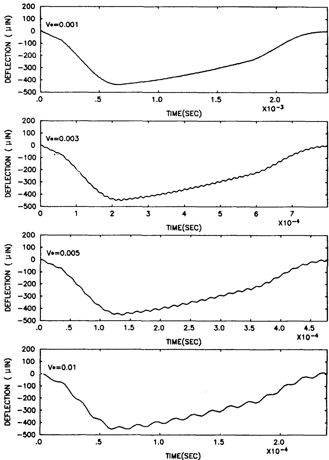
Figure 4-17: Wallace- Seireg loading
