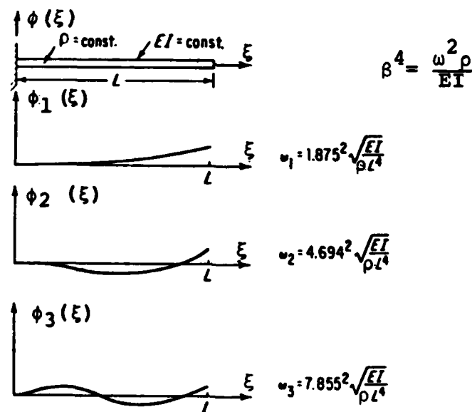
Figure 5-18: Natural Modes
