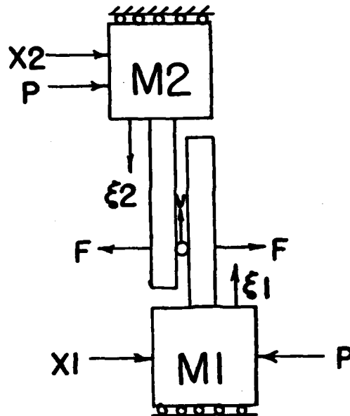
Figure 5-17: System parameters
