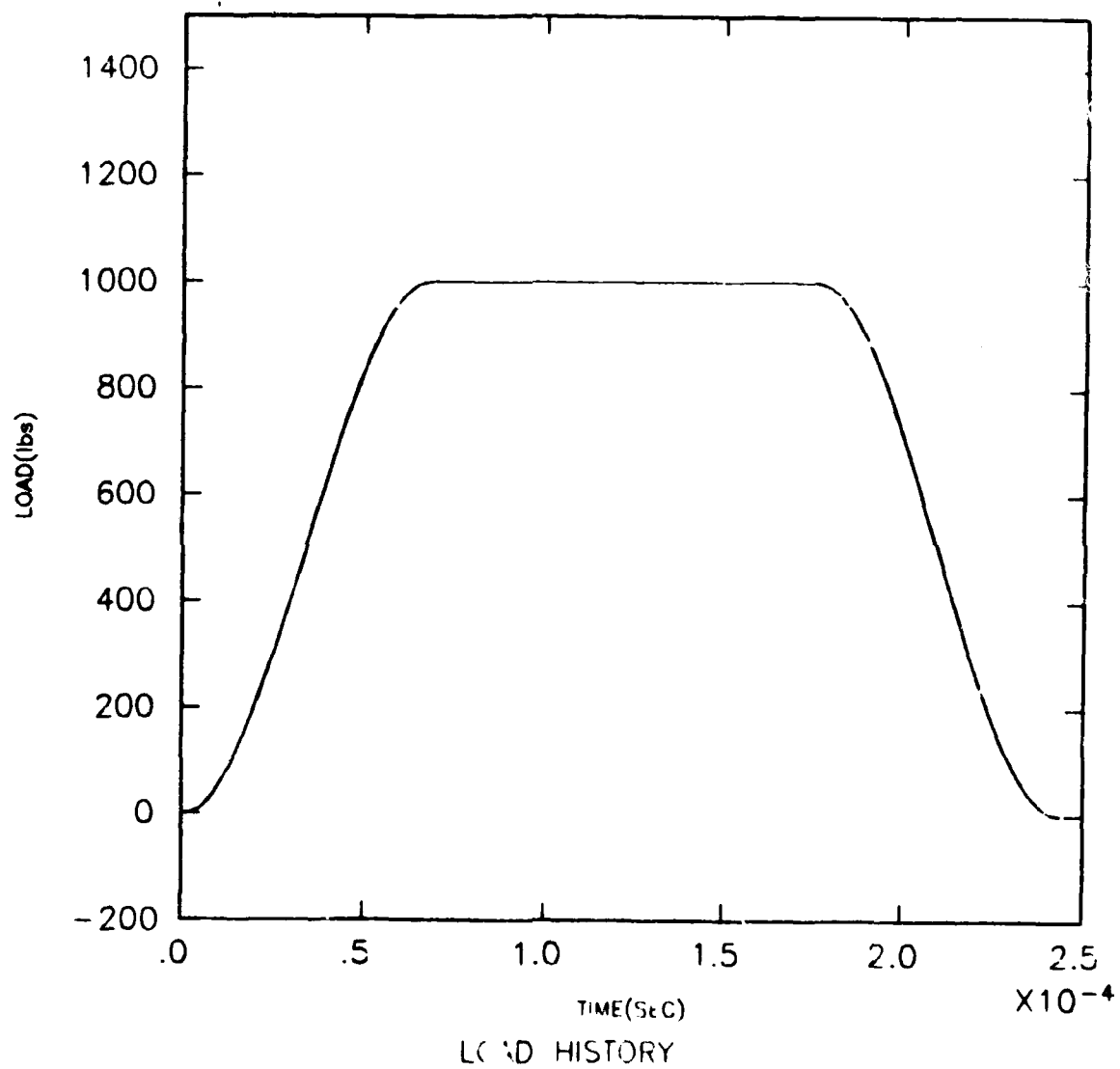
Figure 4-5: Wallace - Seireg loading
