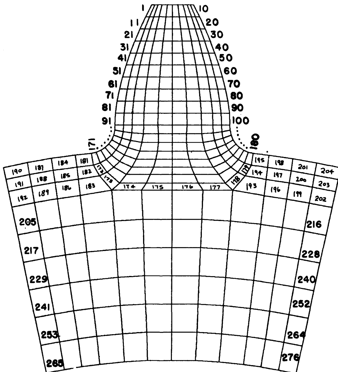
Figure 2-13: Elements
