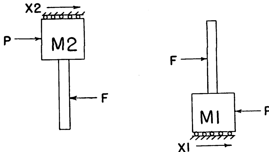
Figure 5-3: Free body diagrams
