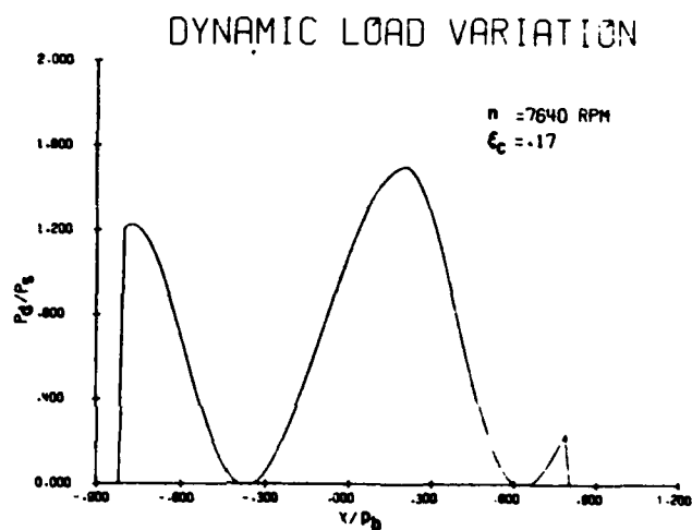
(b) Dynamic Load Variation, r_G = 1 , N_T = 28 , D_p = 8 , D = .254 cm (.1 in.) (a) n = 1637 \text{ RPM} , (b) n = 7640 \text{ RPM} , and (c) n = 16370 \text{ RPM}
