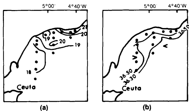
Figure 14. Temperature (a) and salinity (b) at 1 m depth during August 1982 (redrawn from J. Gil, Instituto Español de Oceanografía, Malaga).
