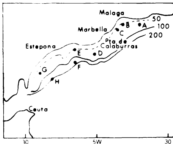
Figure 27. Locations of current meter moorings during 1978-1980
