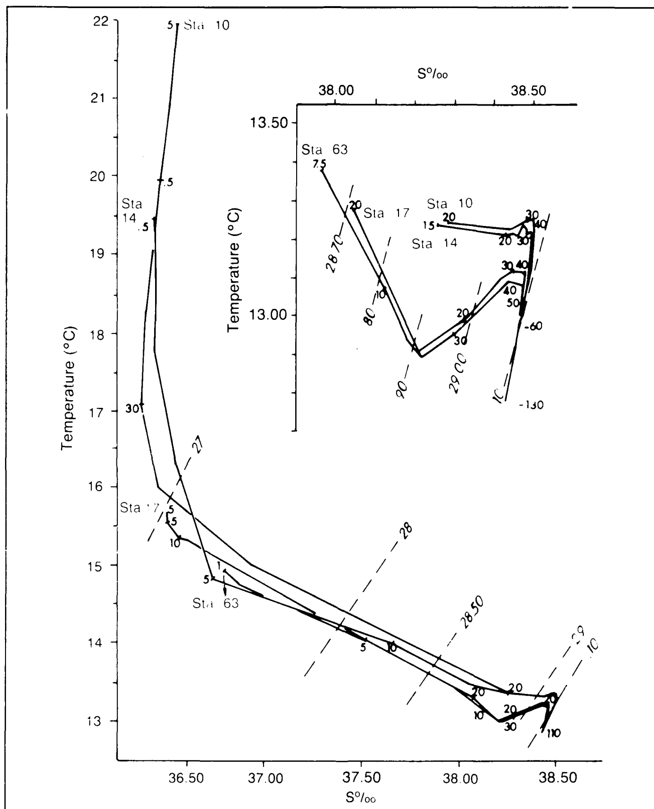
Figure 12. Temperature-salinity curves for the stations shown in Figure 10.
