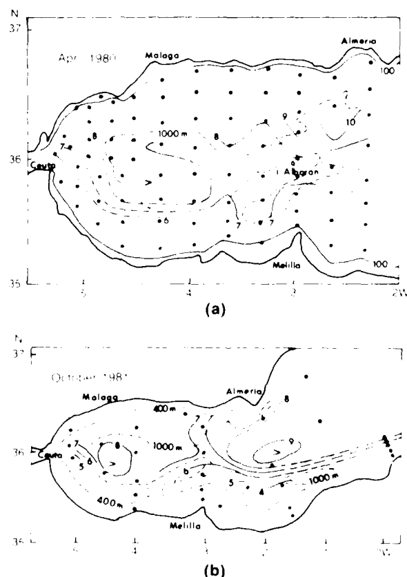
Figure 23. Depths of the 12.90^{\circ}C potential temperature surface (hm) in (a) April 1980 and (b) October 1981.
