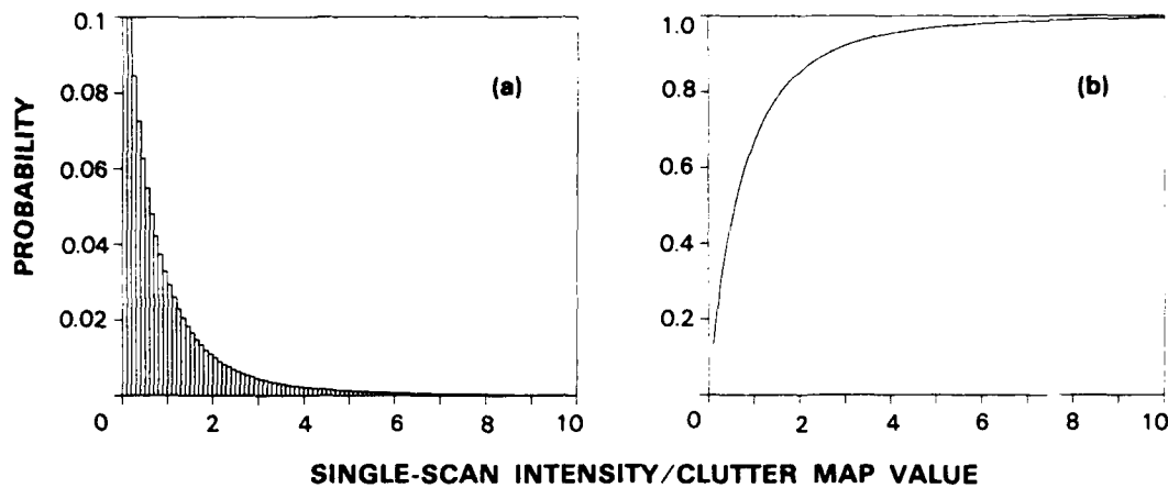
Figure III-5. Composite clutter fluctuation distributions. Data from Figures III-3 and III-4 are combined (Equation 7 in the text) to compute the distribution of single-scan clutter intensity to a scan-averaged value measured as much as two weeks earlier. (a) Probability density function; (b) cumulative distribution.
