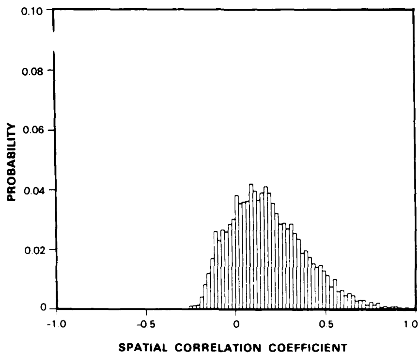
Figure III-7. Distribution of cross-correlation coefficients for intensity fluctuations in resolution cells within the spatial filter window. This histogram is from all 9-cell nearest neighbor clusters within 12 km of the testbed ASR.
