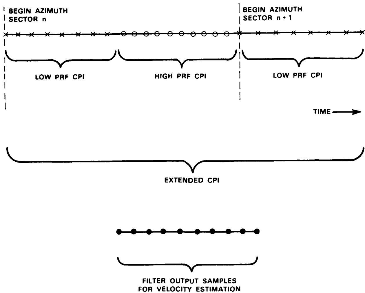
Figure II-2. Illustration of multiple-CPI clutter filtering technique.
