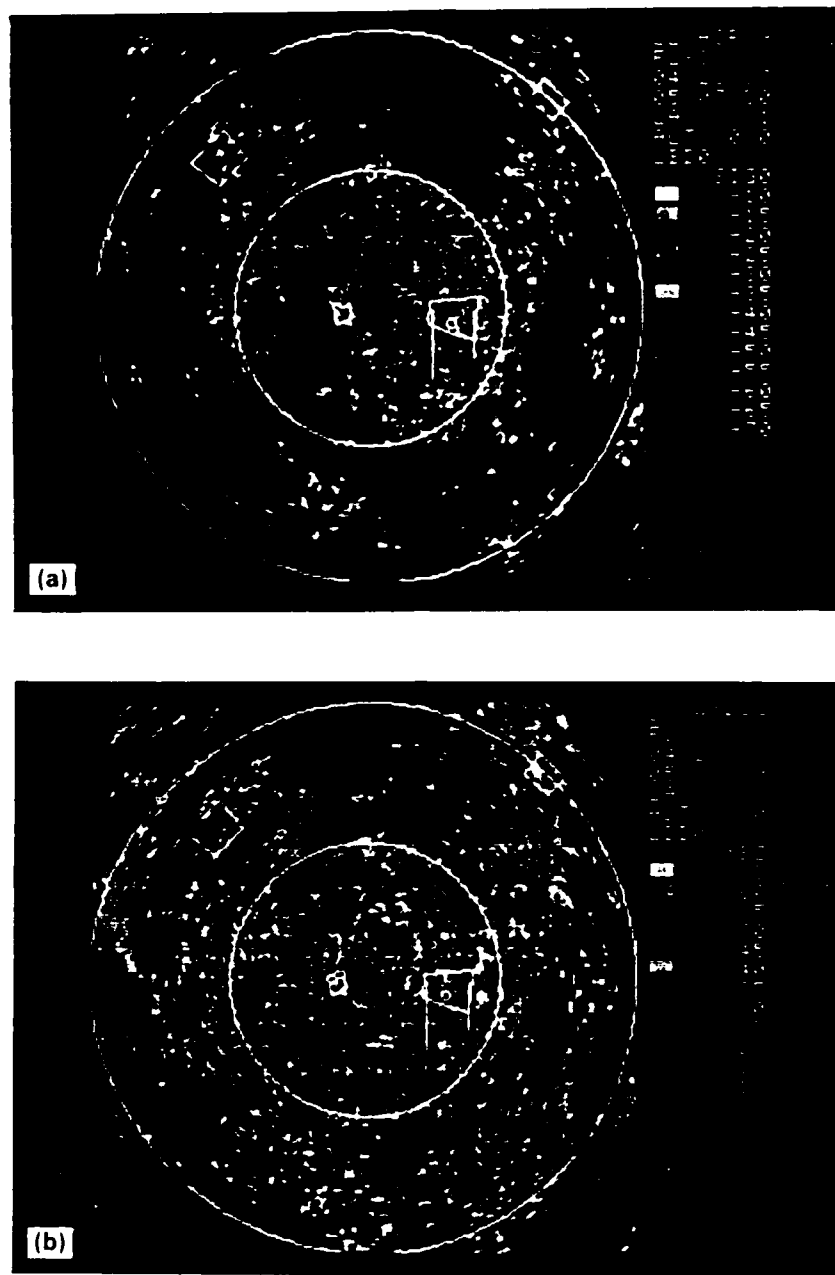
Figure III-2. (a) Display of ground clutter cross section density \sigma_0 from the testbed ASR. The white boxes show areas for analysis of clutter intensity fluctuations: (1) Rainbow Mountain (northeast at 10 km); (2) Huntsville Airport (east at 3 km); (3) Wildlife Refuge (west at 1.5 km); (4) Limestone Creek area (northwest at 8 km); North-south oriented parallel lines indicate the runways at Huntsville Airport; (b) display of the equivalent weather reflectivity factor of ground clutter from the testbed ASR.
