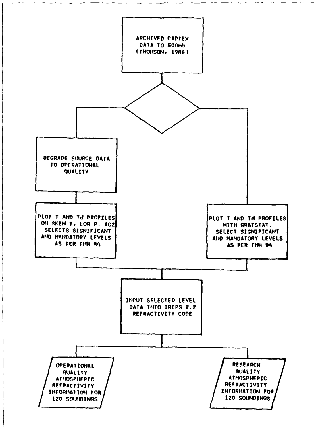
Fig. 4.8 Flow diagram of CAPTEX data processing steps.
