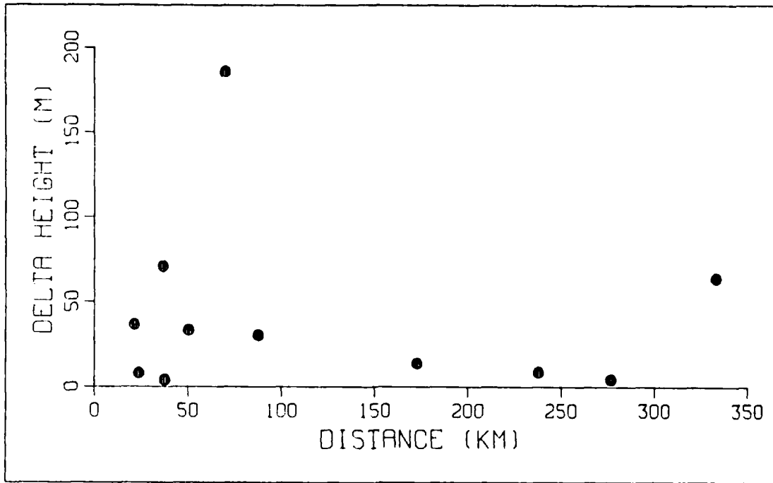
Fig. 5.11 Differences in 50% POD lobe 4 heights for a SPS-10 radar.
