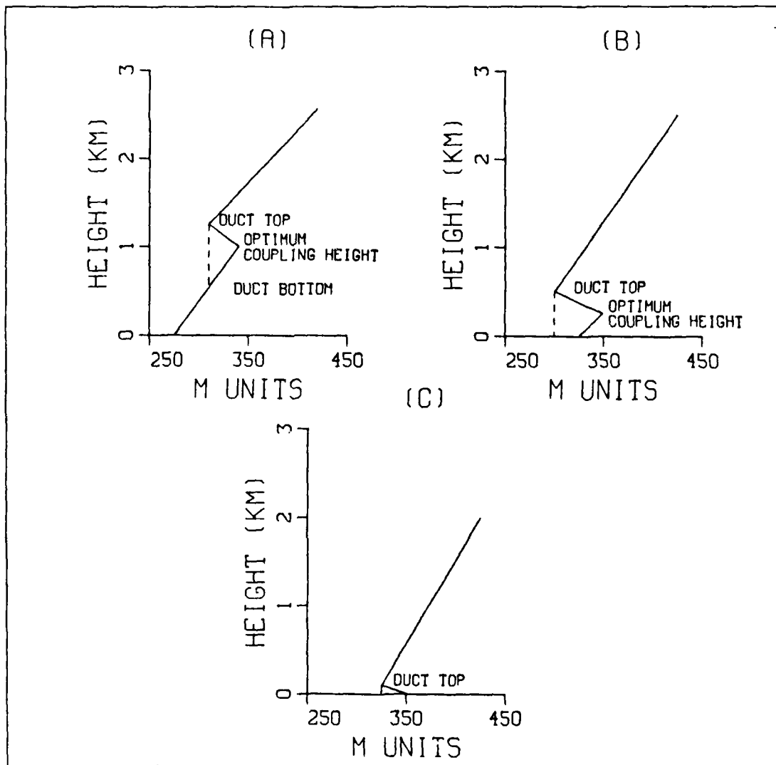
Fig. 2.1 Ducting occurrences for typical M profiles.
