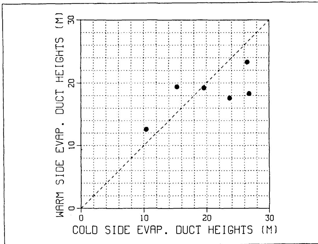
Fig. 5.6 Cold side versus warm side duct heights.
