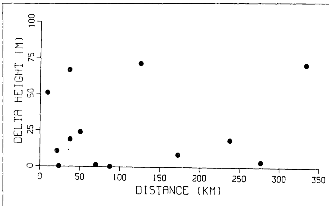
Fig. 5.8 Differences in 50% POD lobe 1 heights for a SPS-10 radar.
