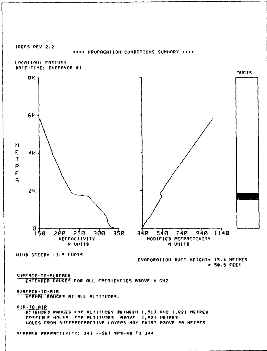
Fig. 3.2 IREPS propagation conditions summary for R/V Endeavor launch number 1.
