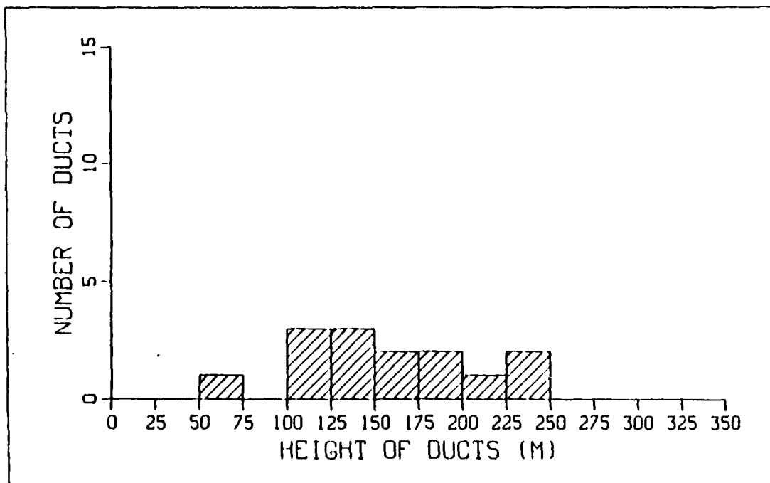
Fig. 5.3 Histogram of CAPTEX low resolution data duct heights.
