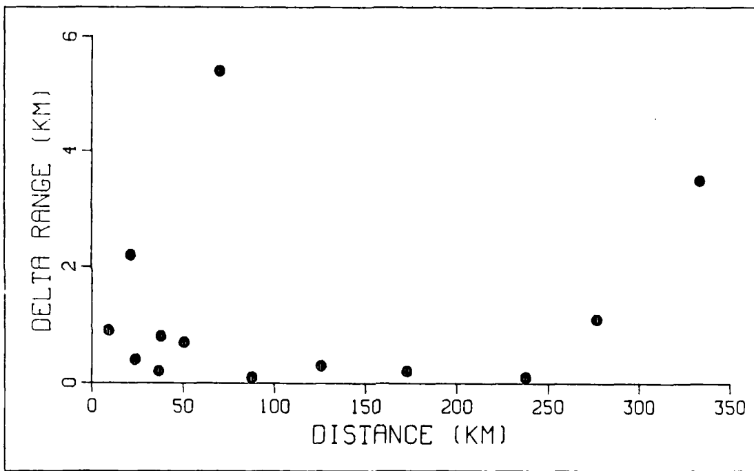
Fig. 5.15 Differences in 50% POD lobe 4 ranges for a SPS-10 radar.
