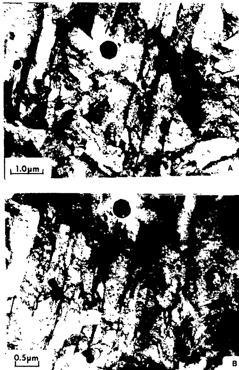
Figure 33. TEM Micrograph of W125 A.) Inclusion and Laths and Retained Austenite in the Weld Metal B.) Inclusions, Laths in Weld Metal
