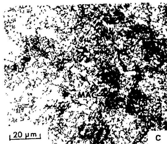
Figure 29. Micrographs of W119 ( 20.4^{\circ}\text{C}/\text{sec} ) (A.) 301 Vickers Hardness [HV] (B.) 271 HV (C.) 265 HV (D.) 301 HV (E.) 271 HV (F.) 265 HV
