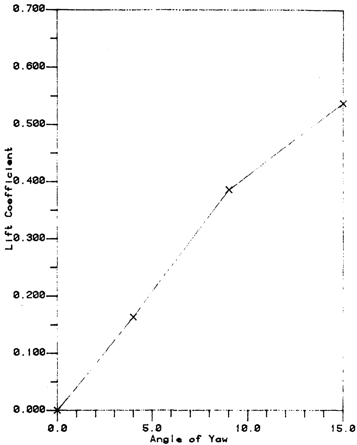
Lift vs Angle of Yaw (Round Tip)
