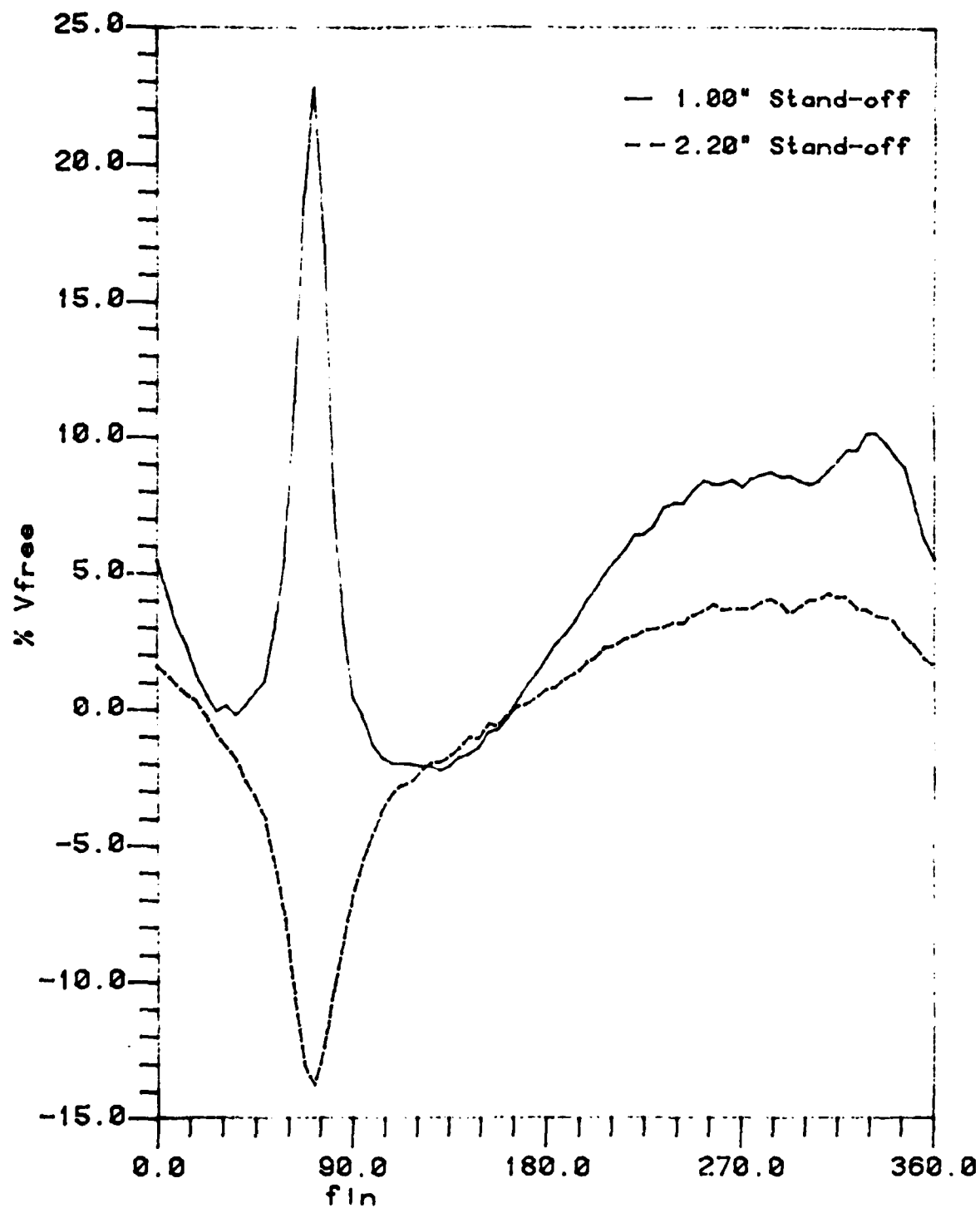
Tangential Velocity vs Body Rotation
