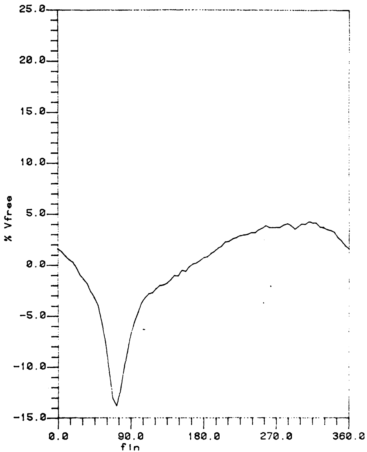
Tangential Velocity vs Body Rotation 2.2" Stand-off
