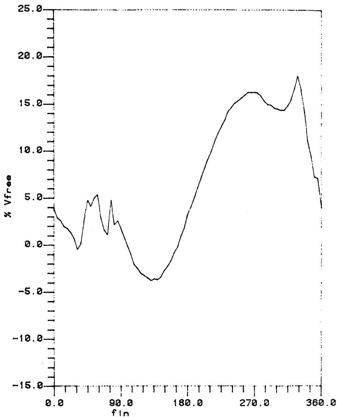
Tangential Velocity vs Body Rotation 0.35" Stand-off
