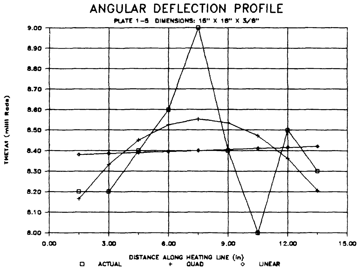
FIGURE 5.6 ANGULAR DEFLECTION PROFILE: PLATE 1-5
