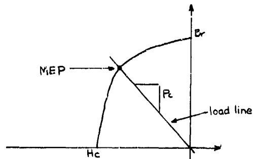
Figure 41. Magnet operating point diagram
