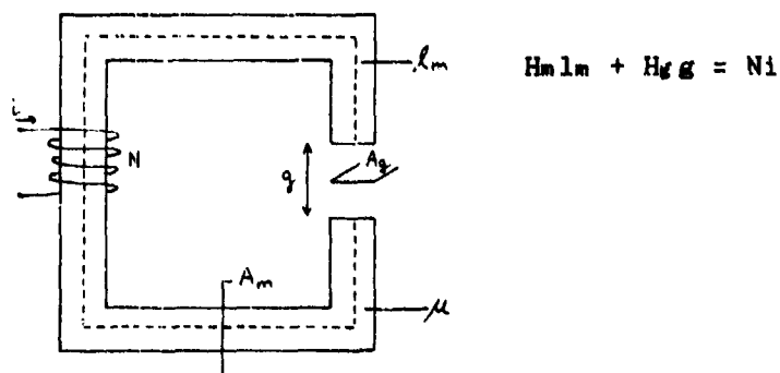
Figure 40. Typical magnetic circuit
