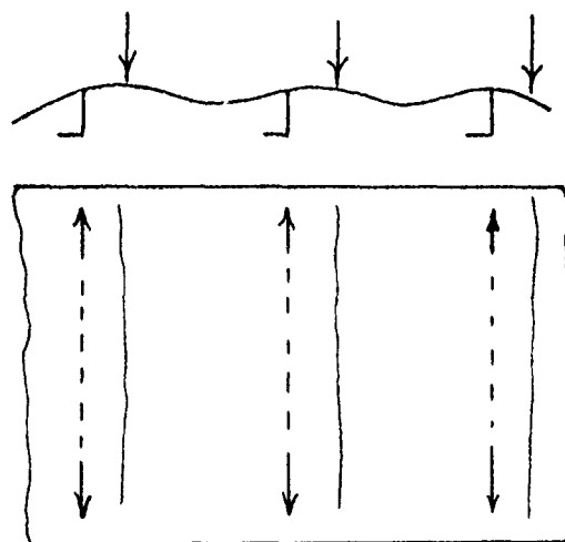
(b) LINE HEATING PANELS
