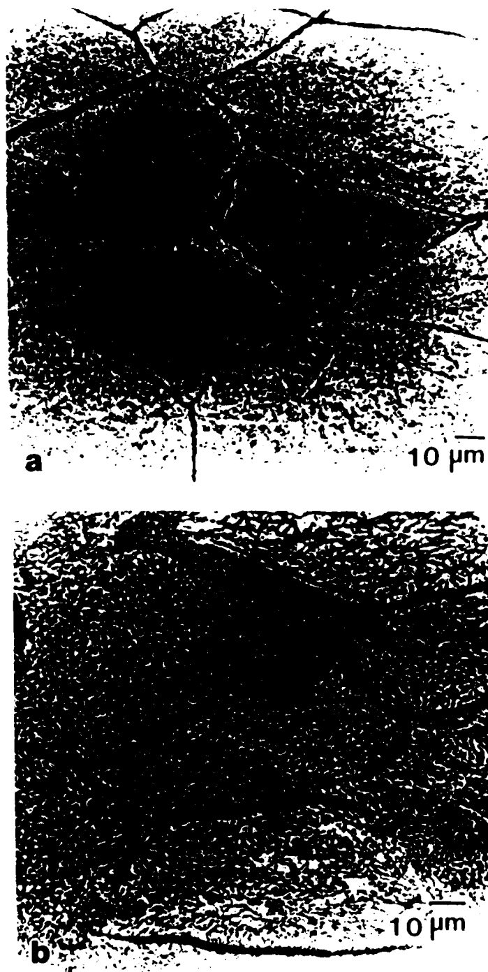
Figure 48. Optical micrographs of the compacts taken perpendicular to the compaction plane. a) Mg-8wt.% Li; b) Mg-8wt.% Li-1.5wt.% Si
